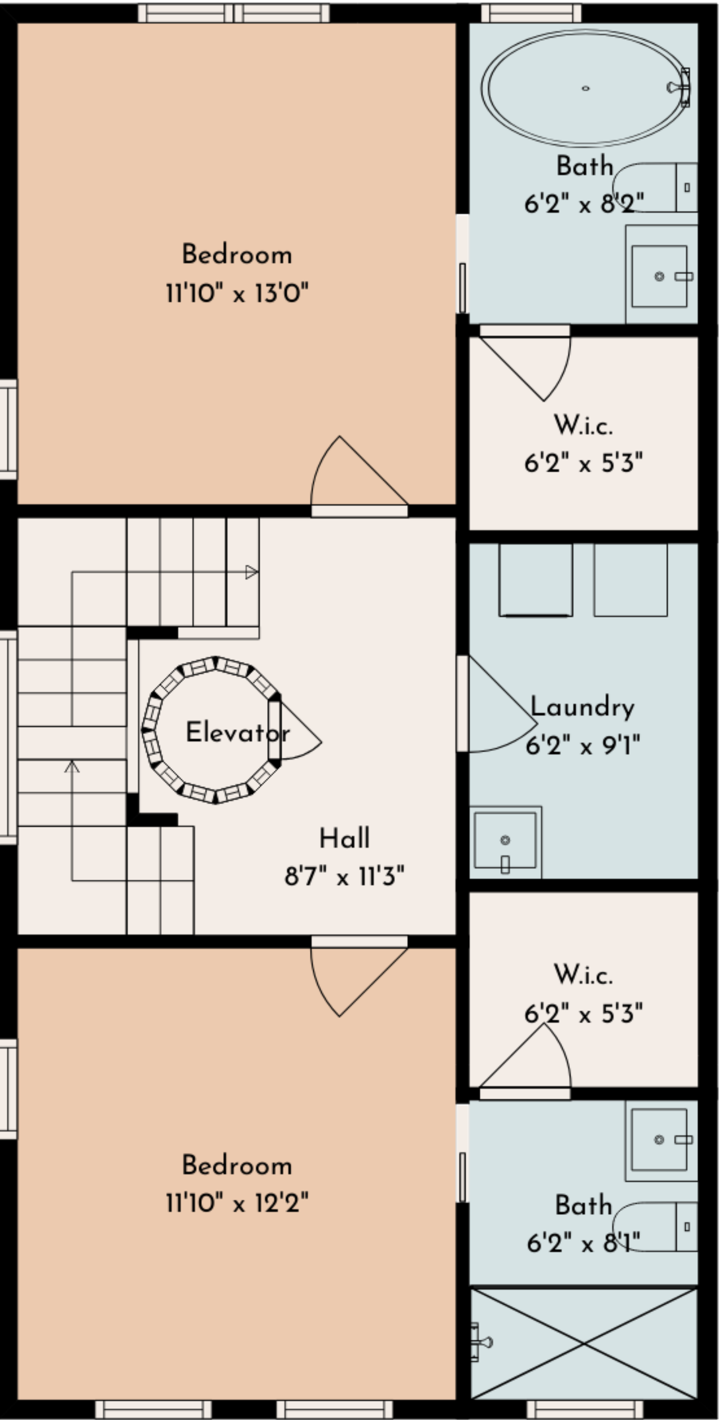
Floor 3
