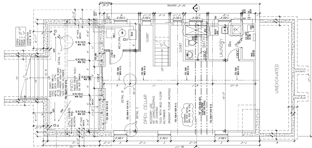
303 CELLAR PLAN SCALE: 1/4"=1'-0"
