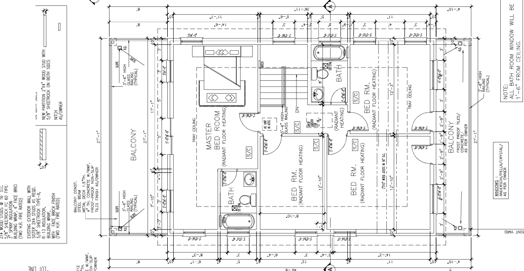
302 SECOND FLOOR PLAN SCALE: 1/4"=1'-0"
