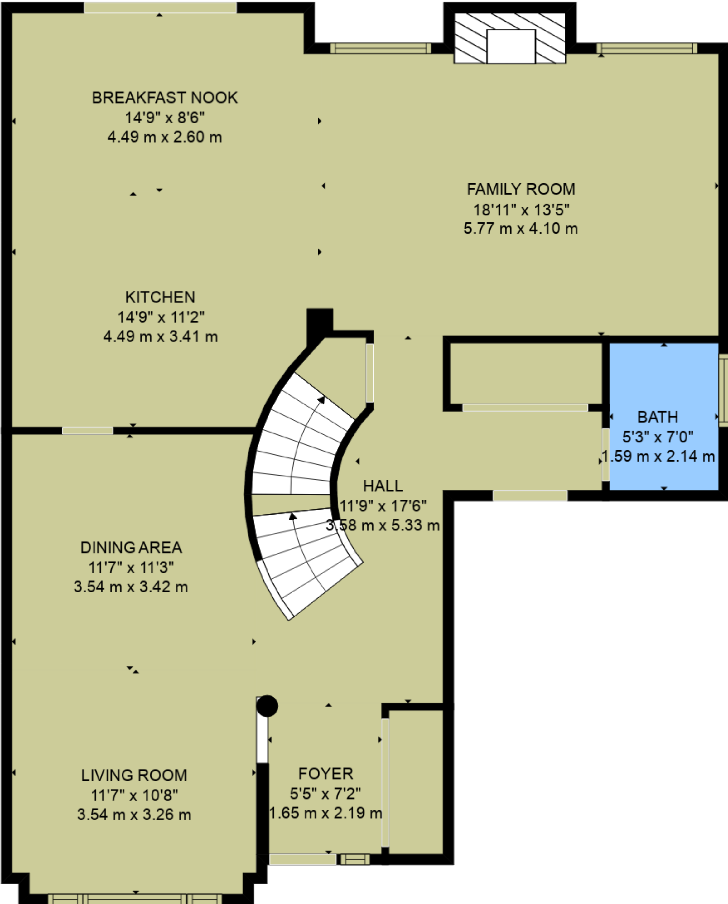
FLOOR 2
