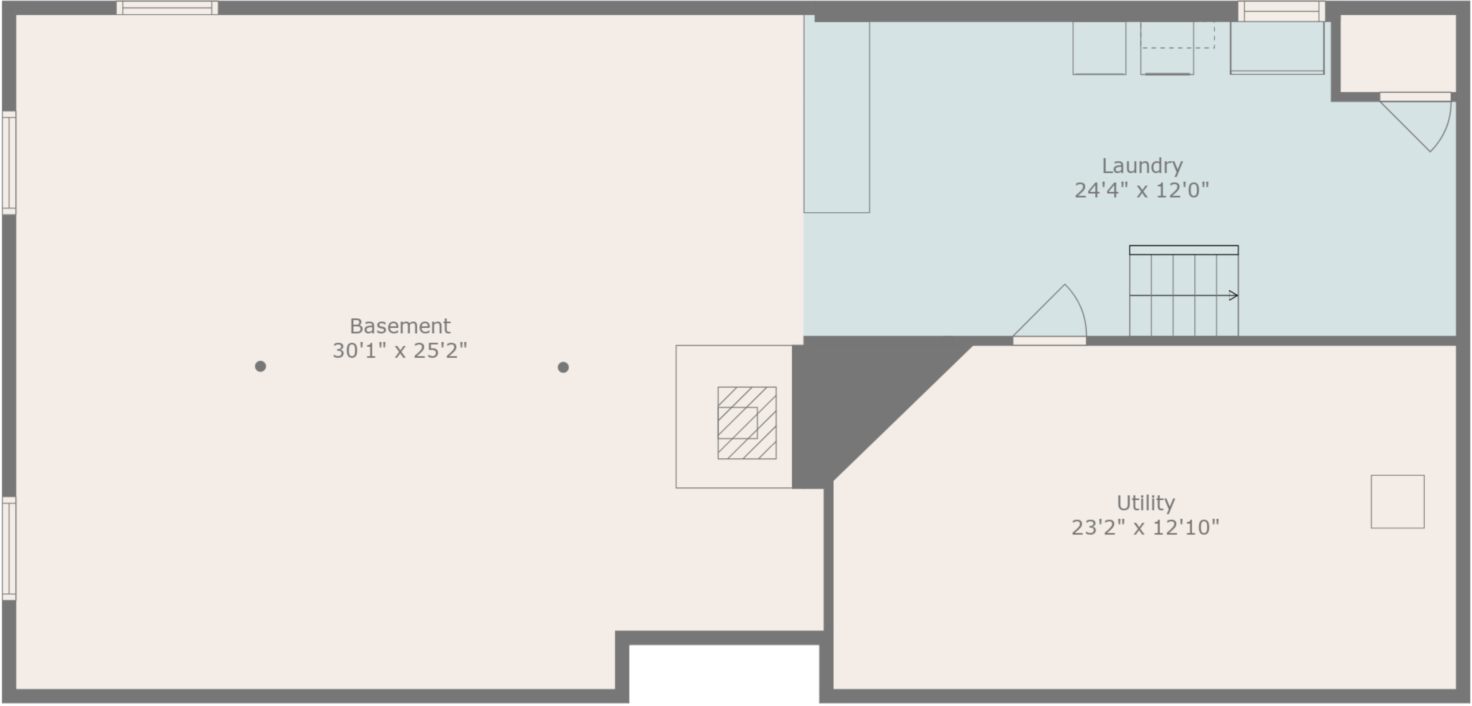
Floor 1
