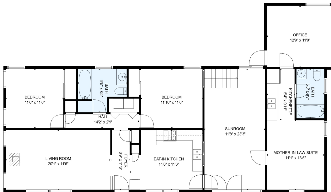
FLOOR 2
