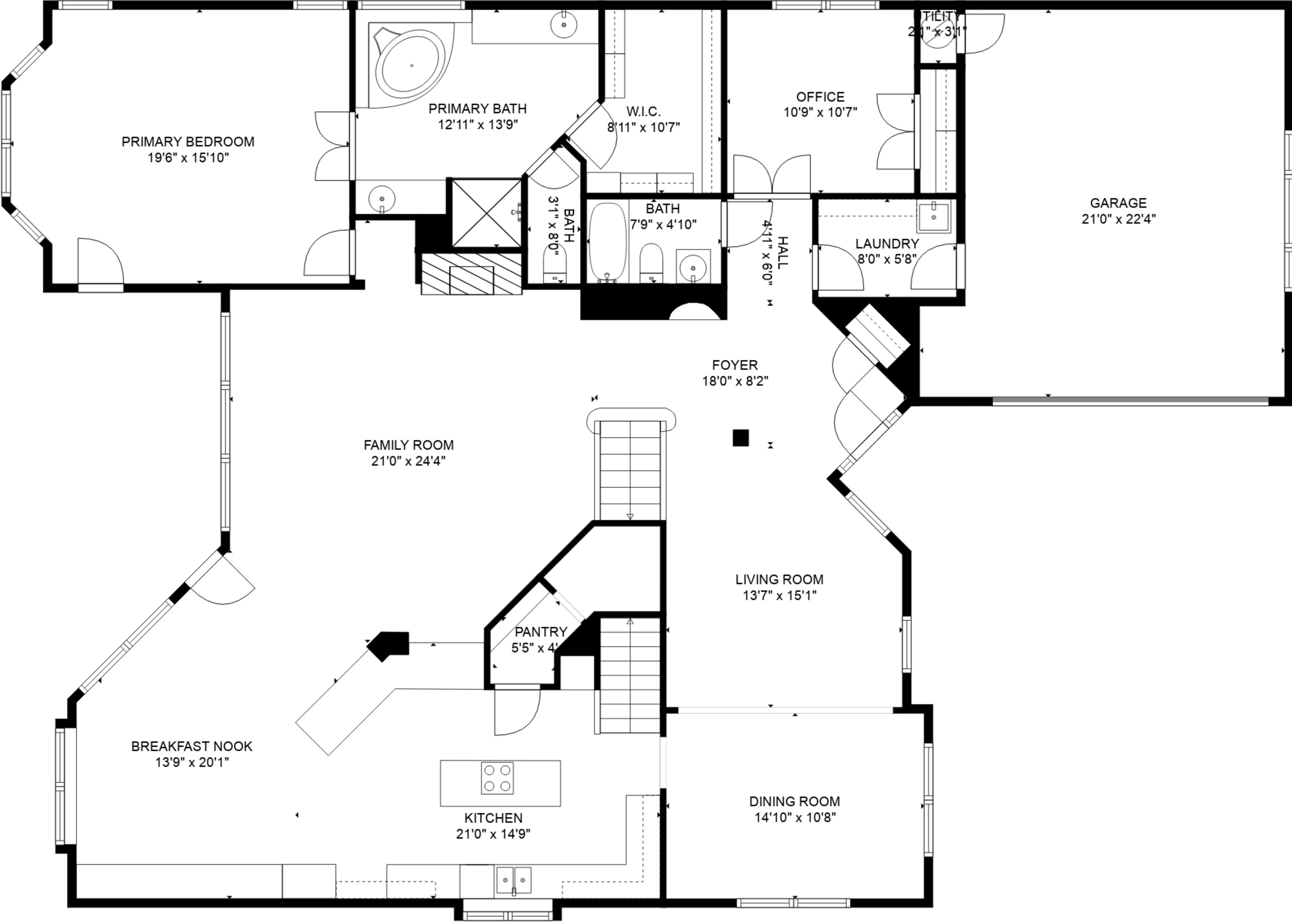
FLOOR 1
