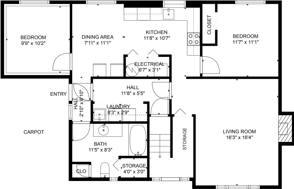
LOWER FLOOR 1,109 SQ.FT.
