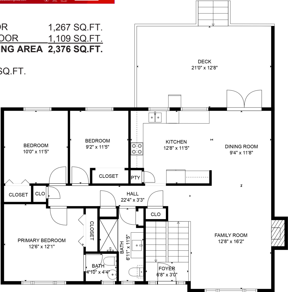
MAIN FLOOR 1,267 SQ.FT.
