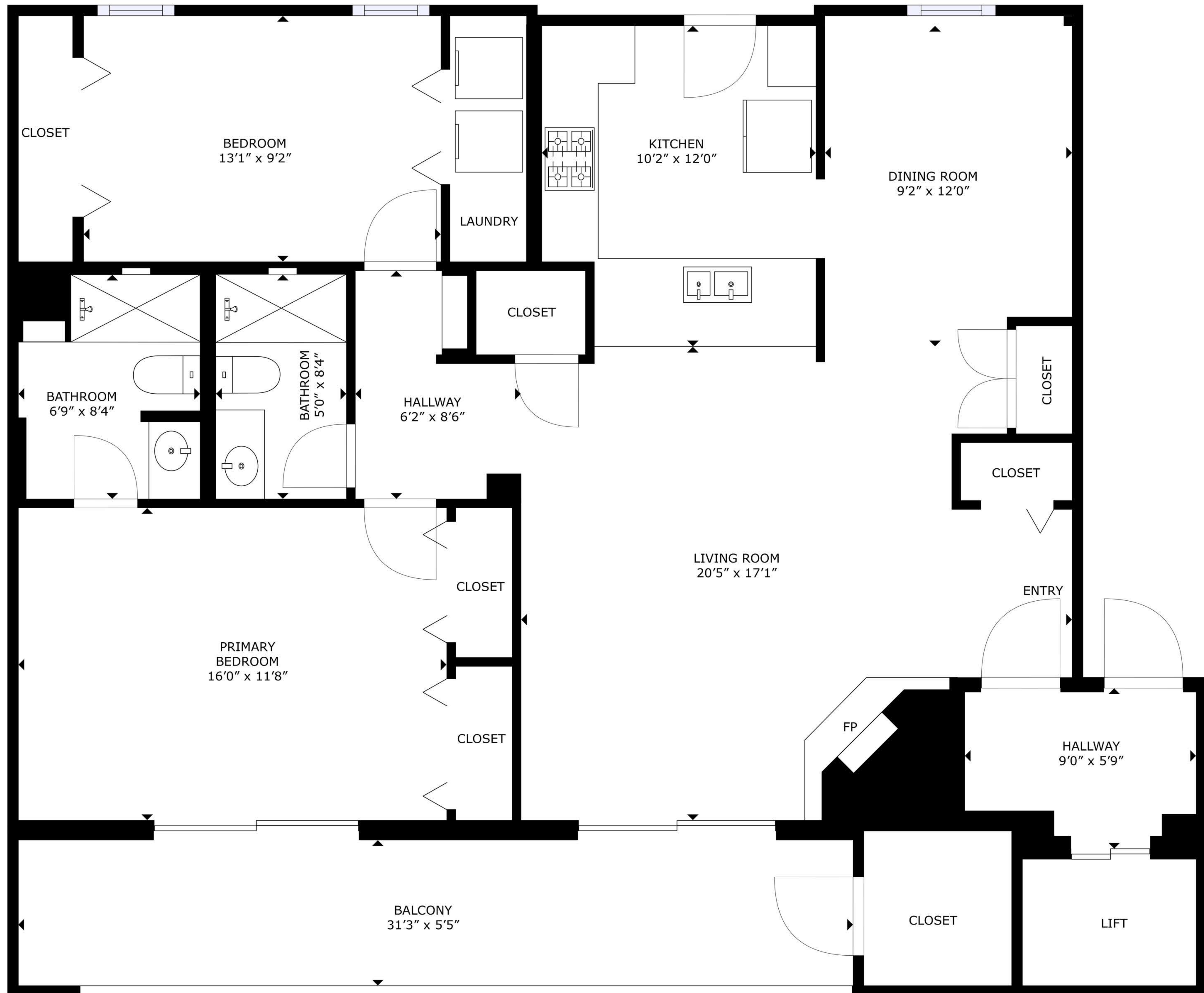
FLOOR PLAN
