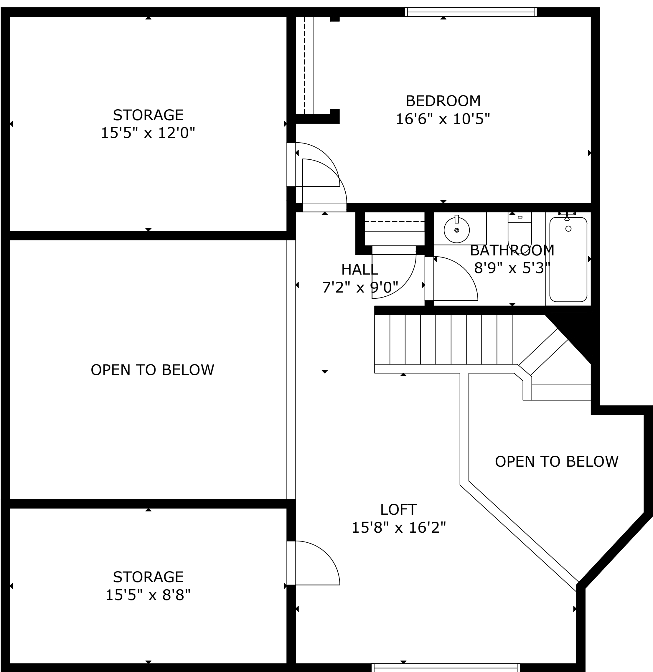
SECOND FLOOR
