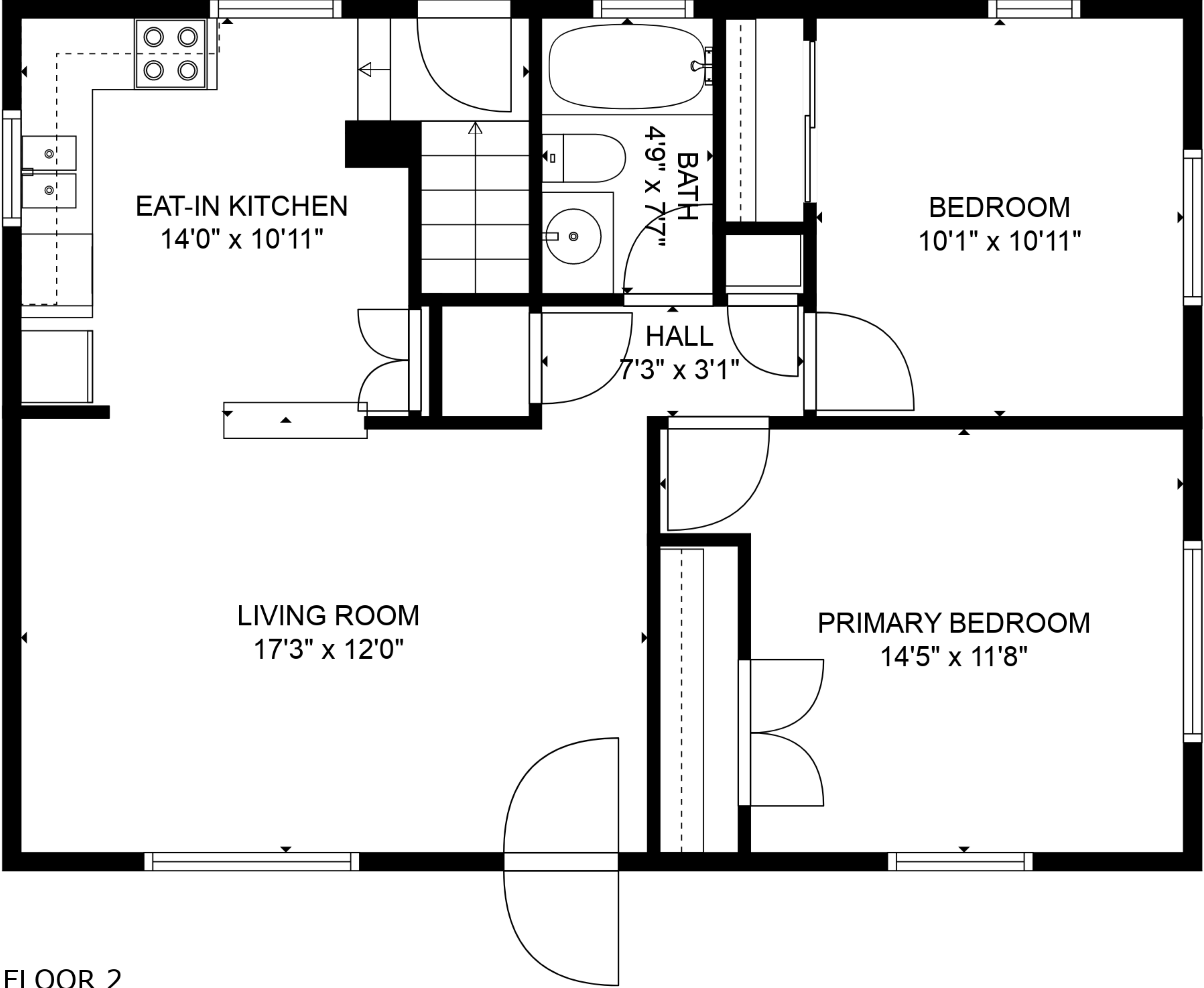
FLOOR 2
