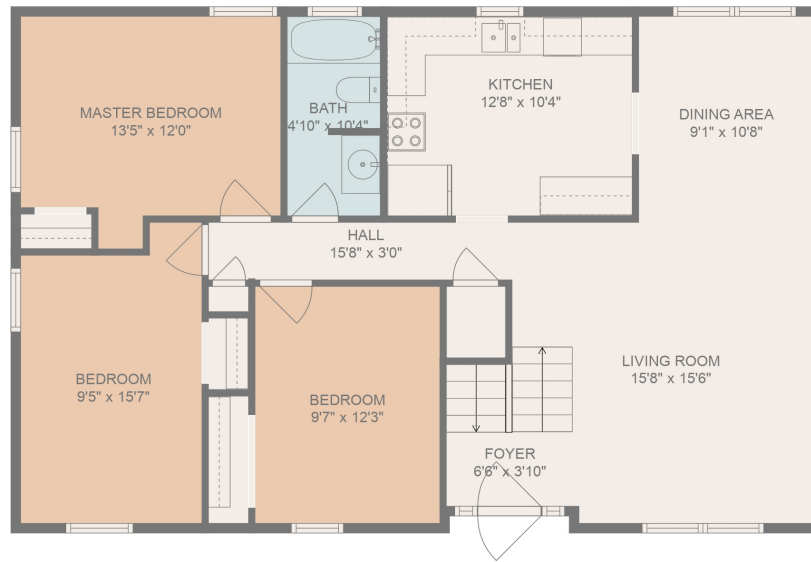
FLOOR 2
