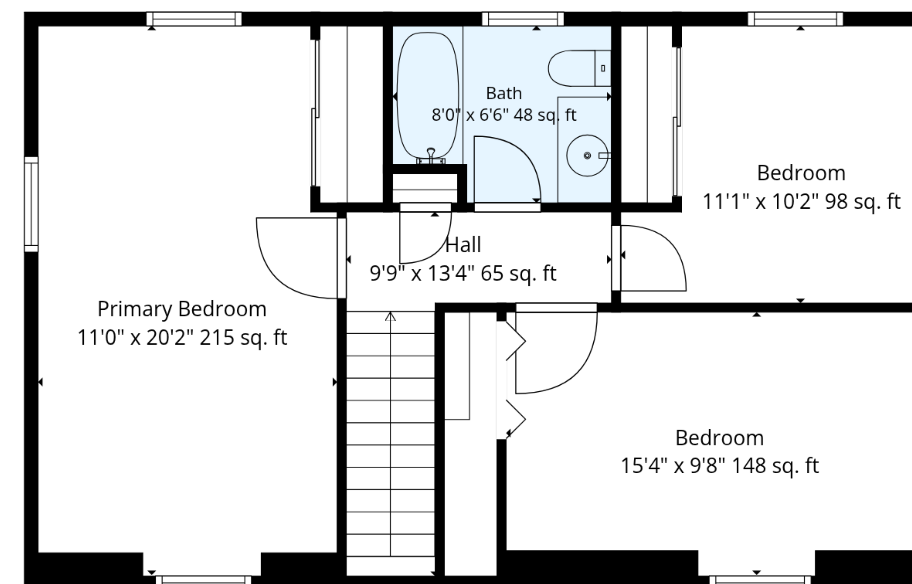
2nd Floor
