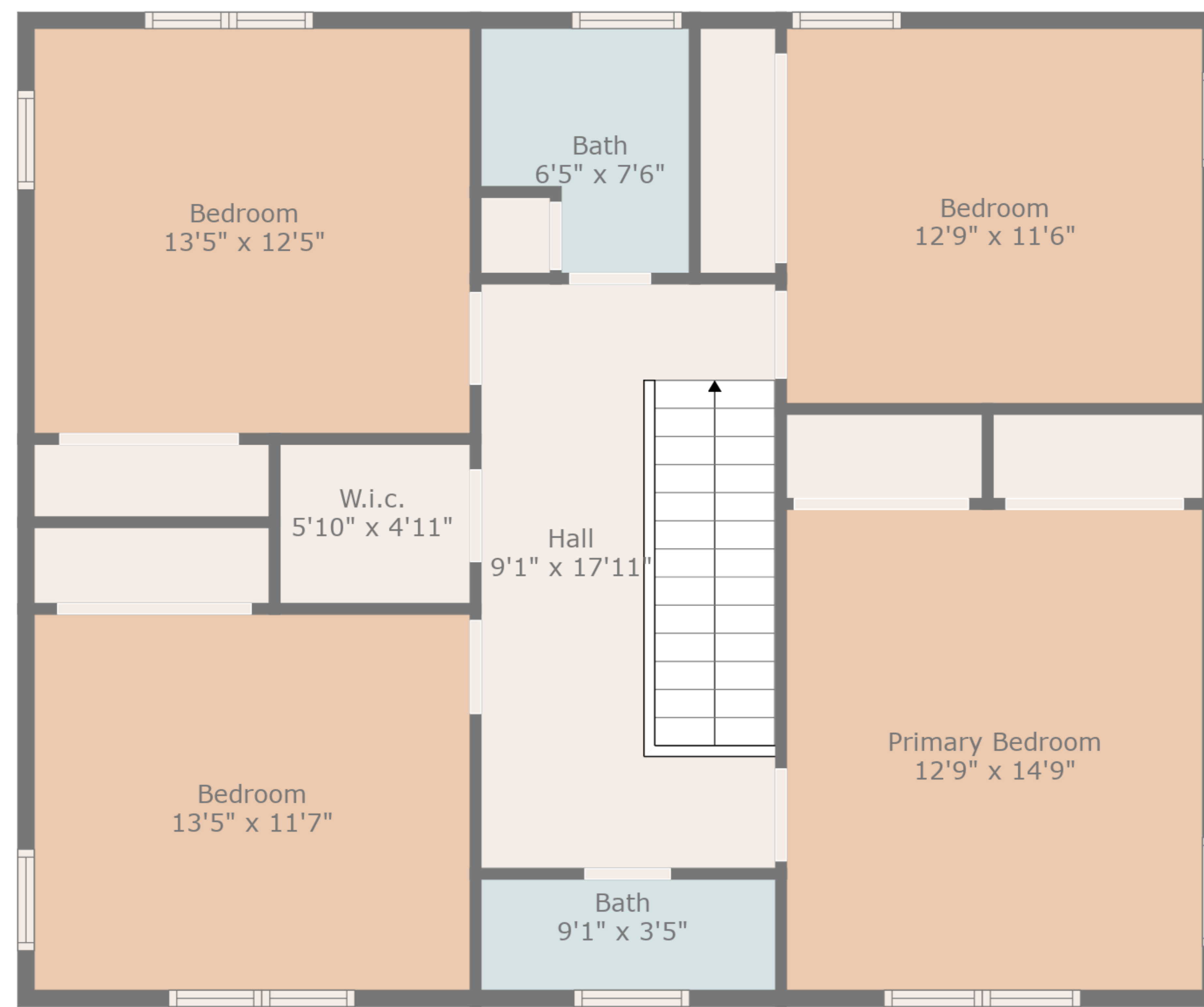
Floor 2
