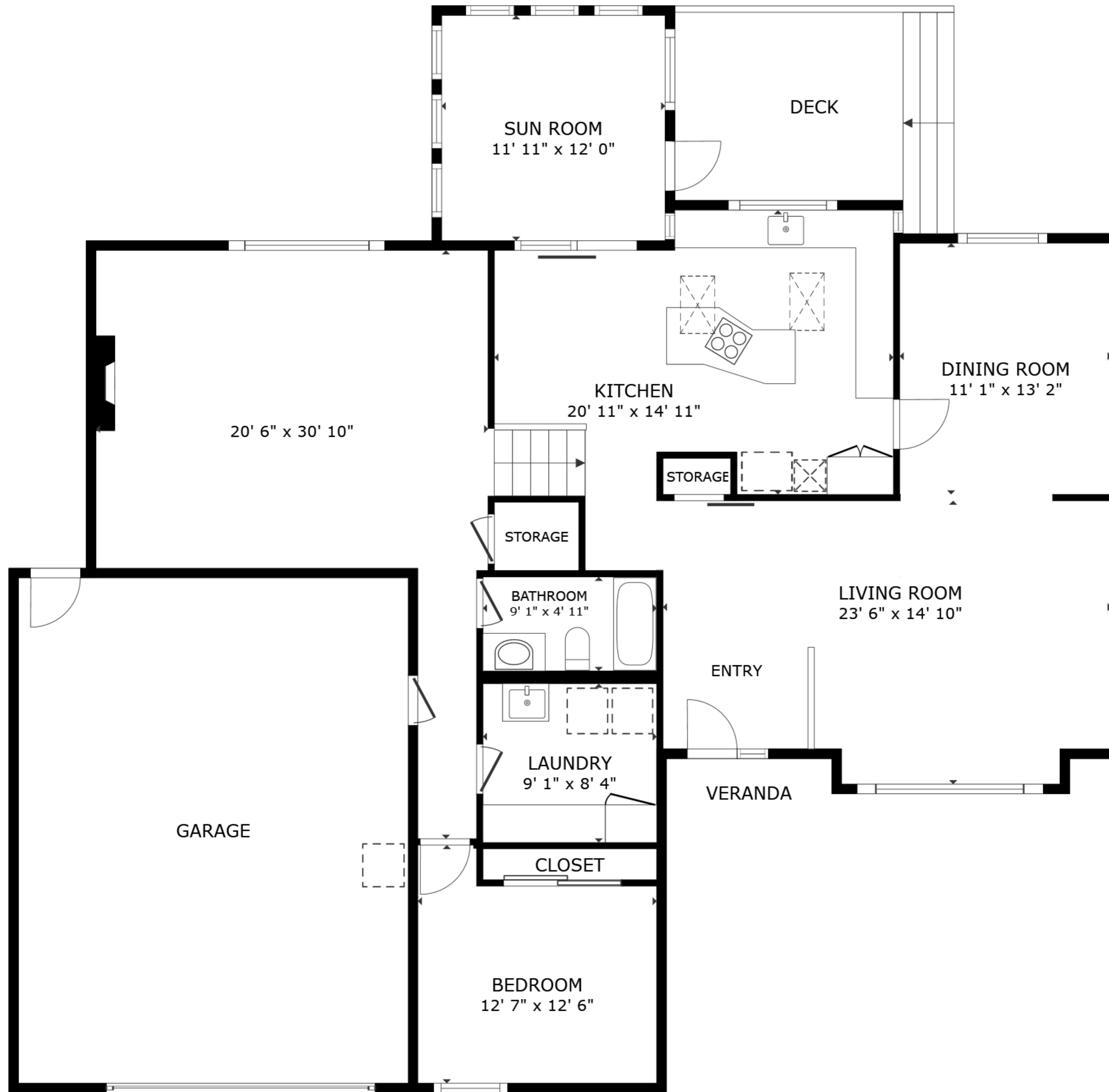
FLOOR 1
