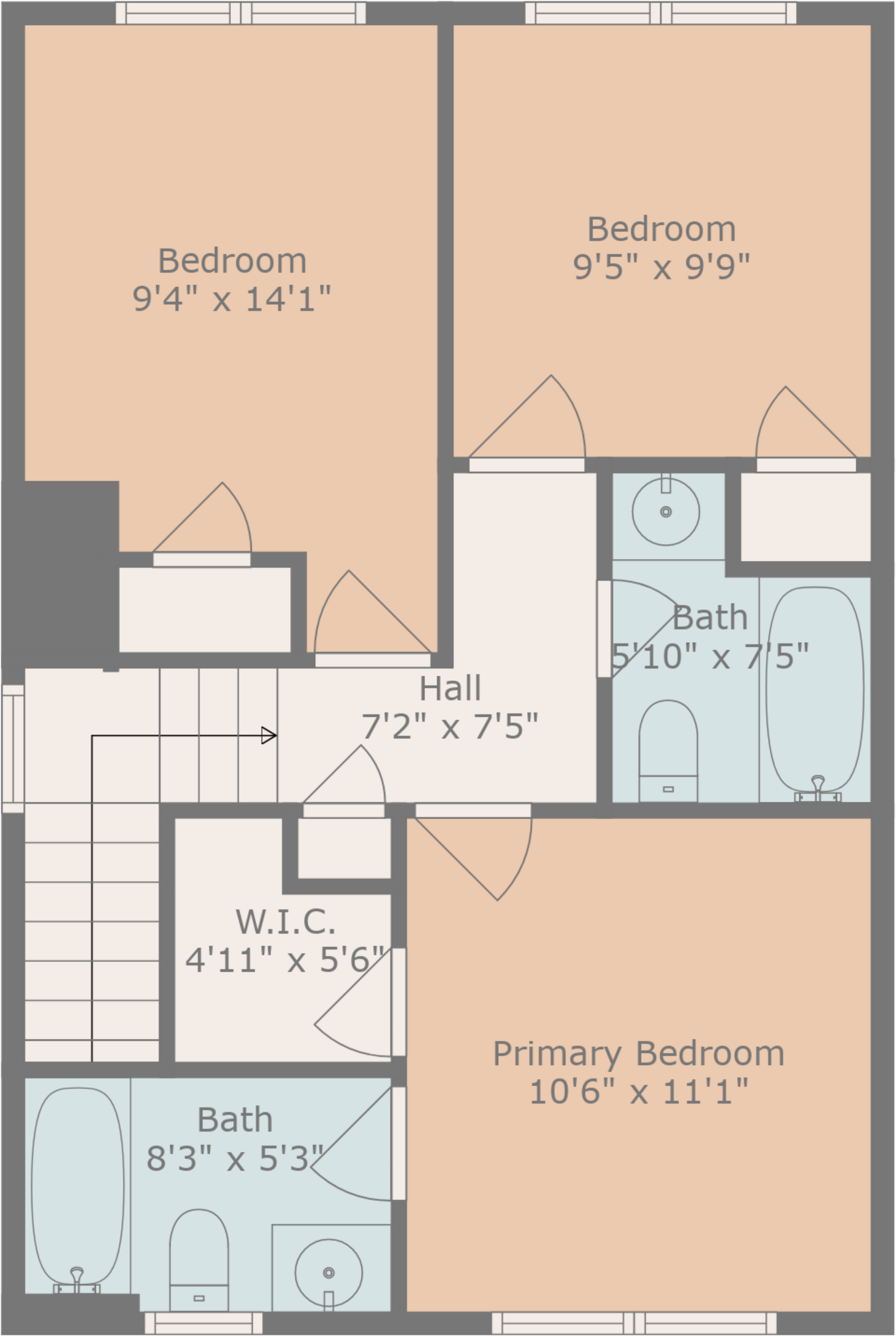
Floor 2
