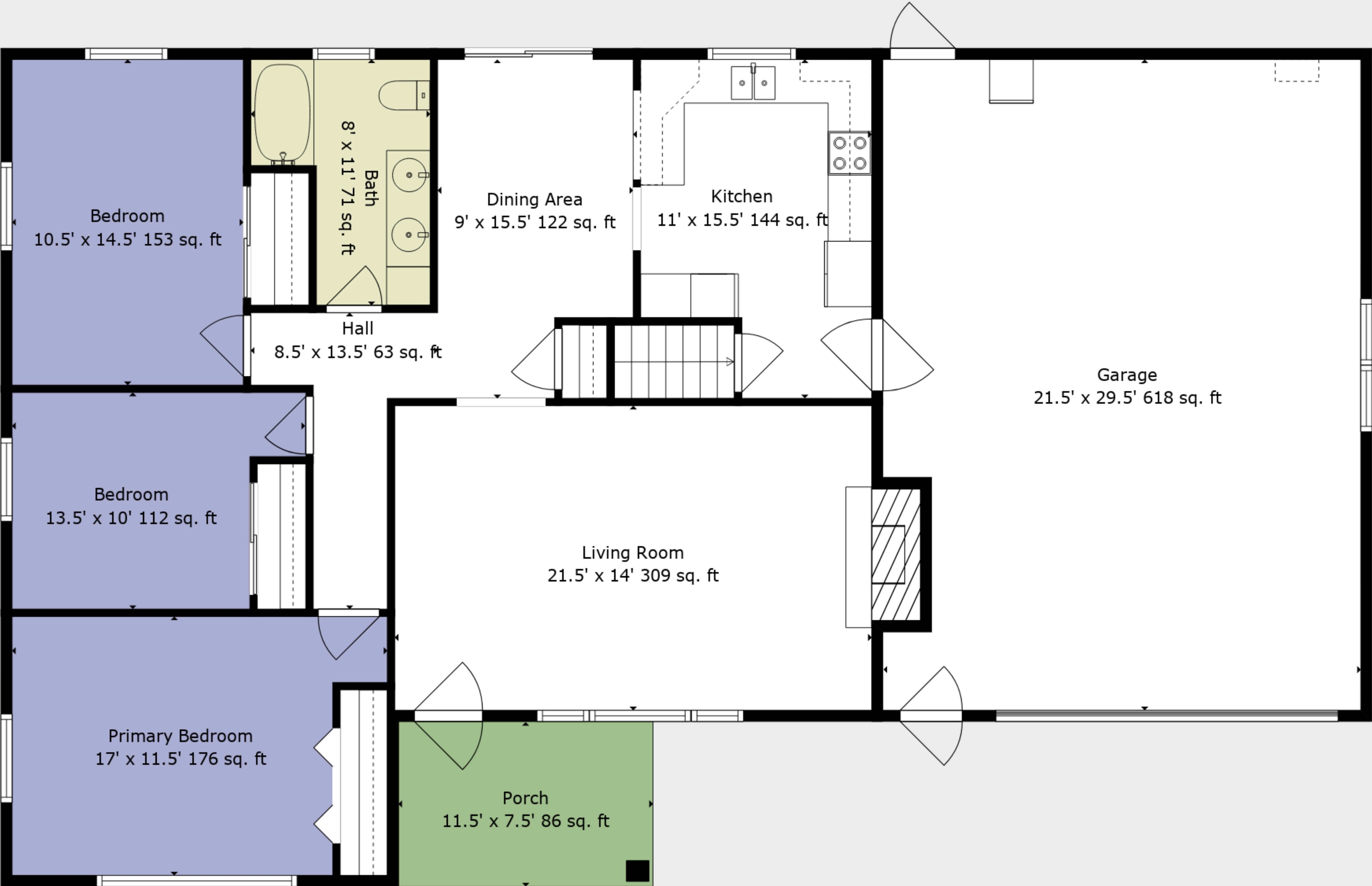
Floor 2
