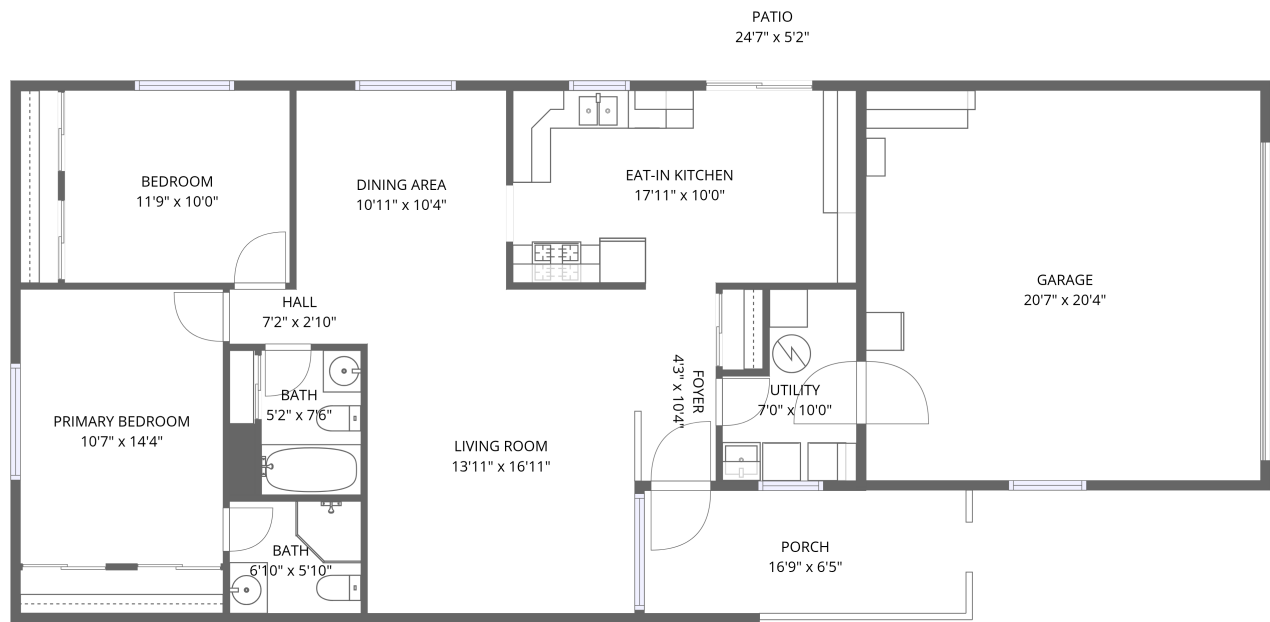
FLOOR 1
