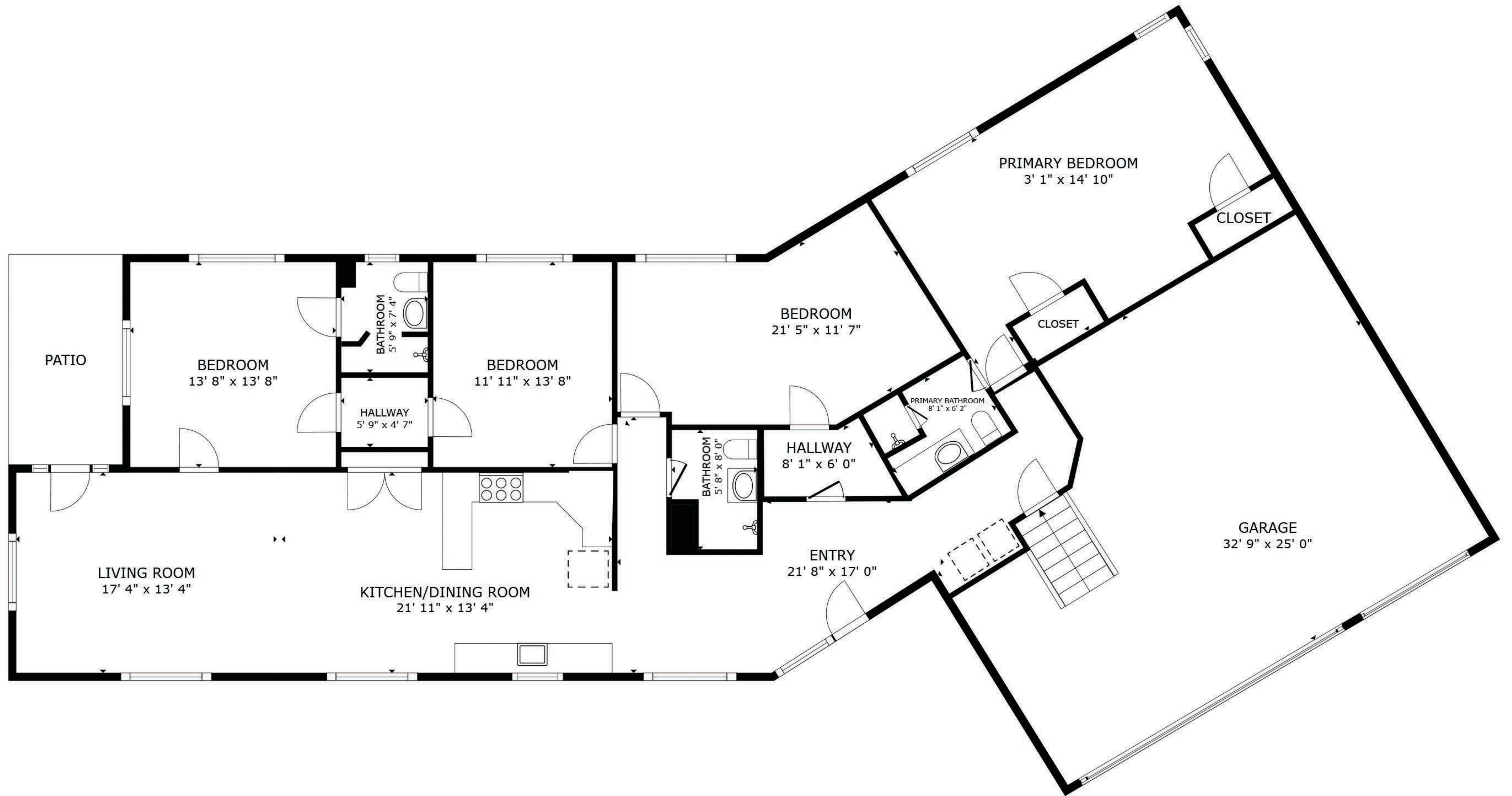
FLOOR PLAN
