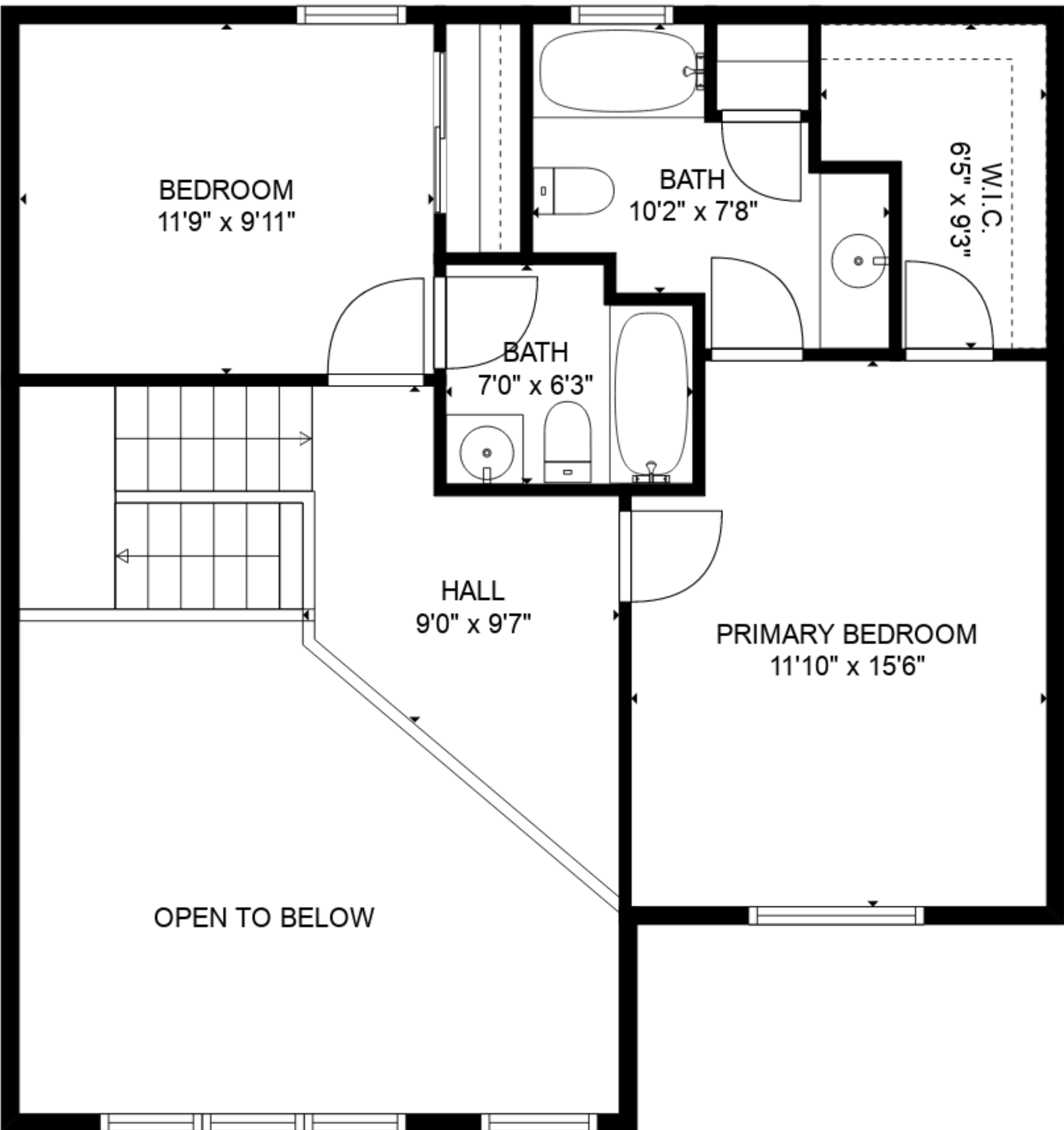
FLOOR 3
