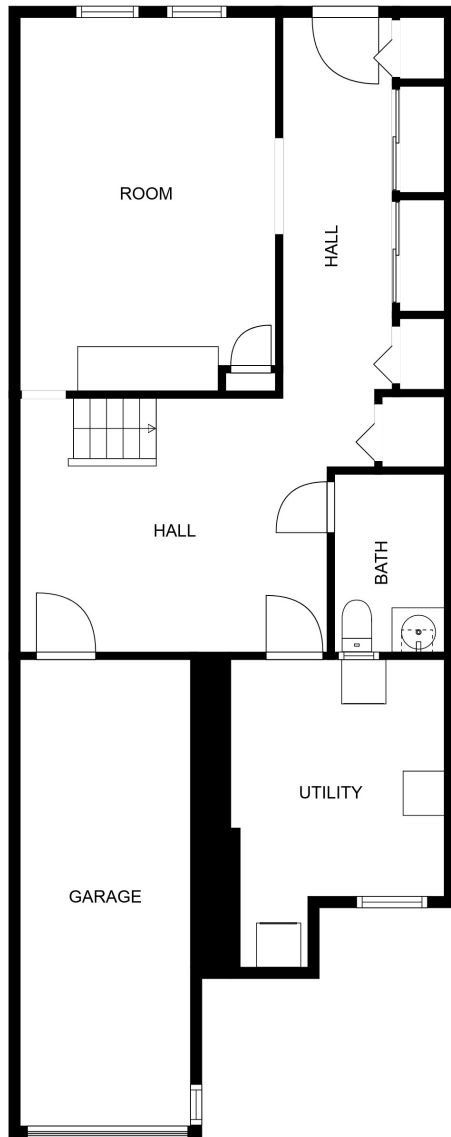
FLOOR 1
