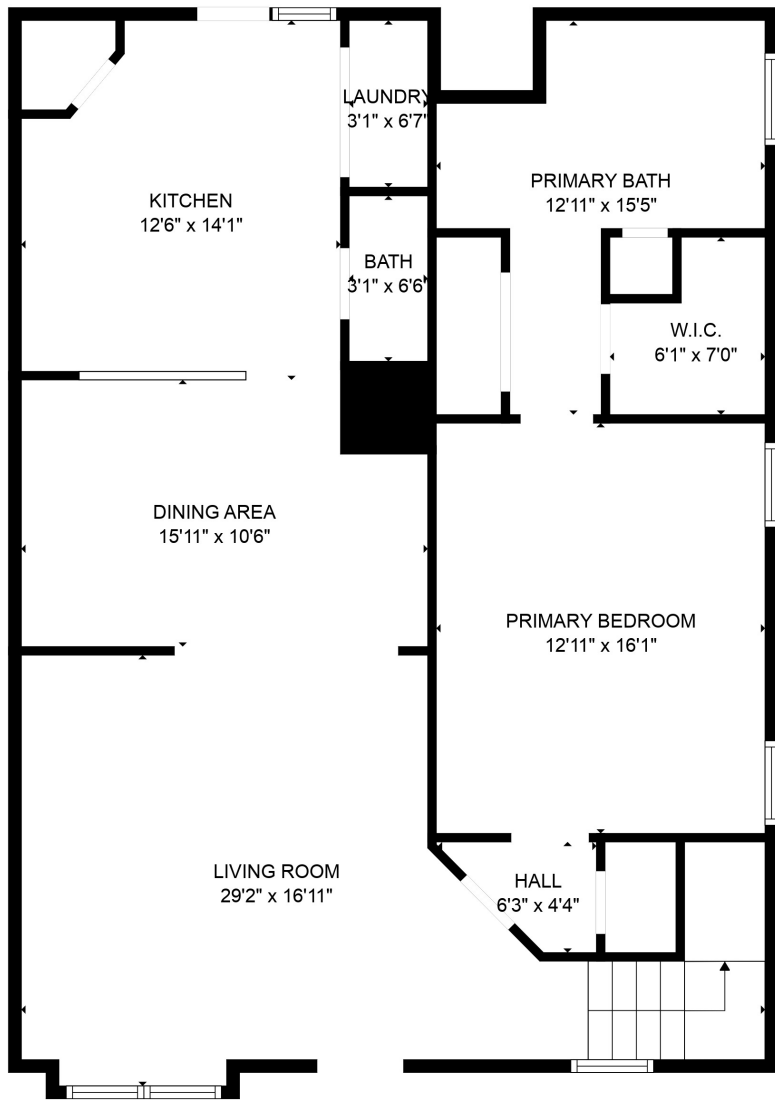
FLOOR 1
