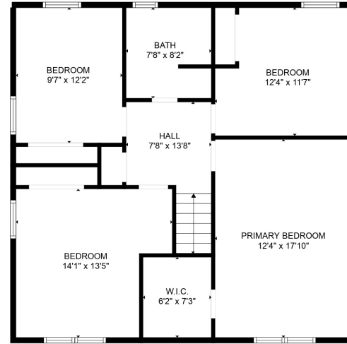
FLOOR 3
