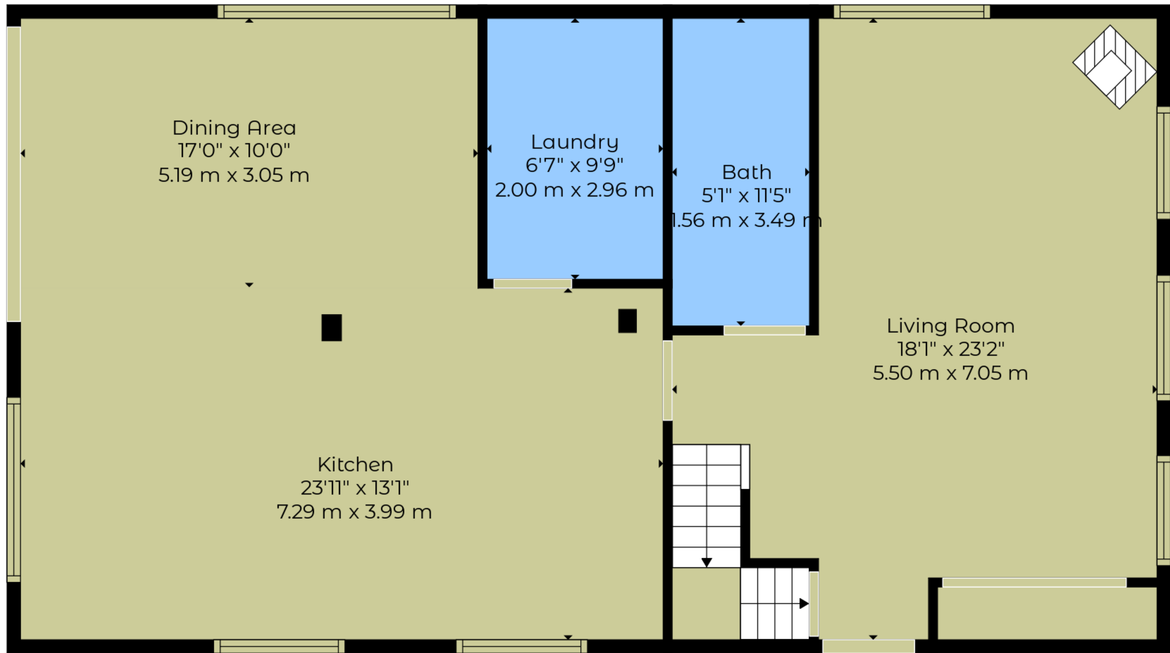
Floor 2
