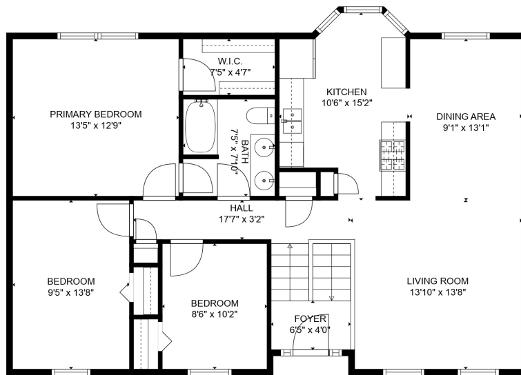
FLOOR 2
