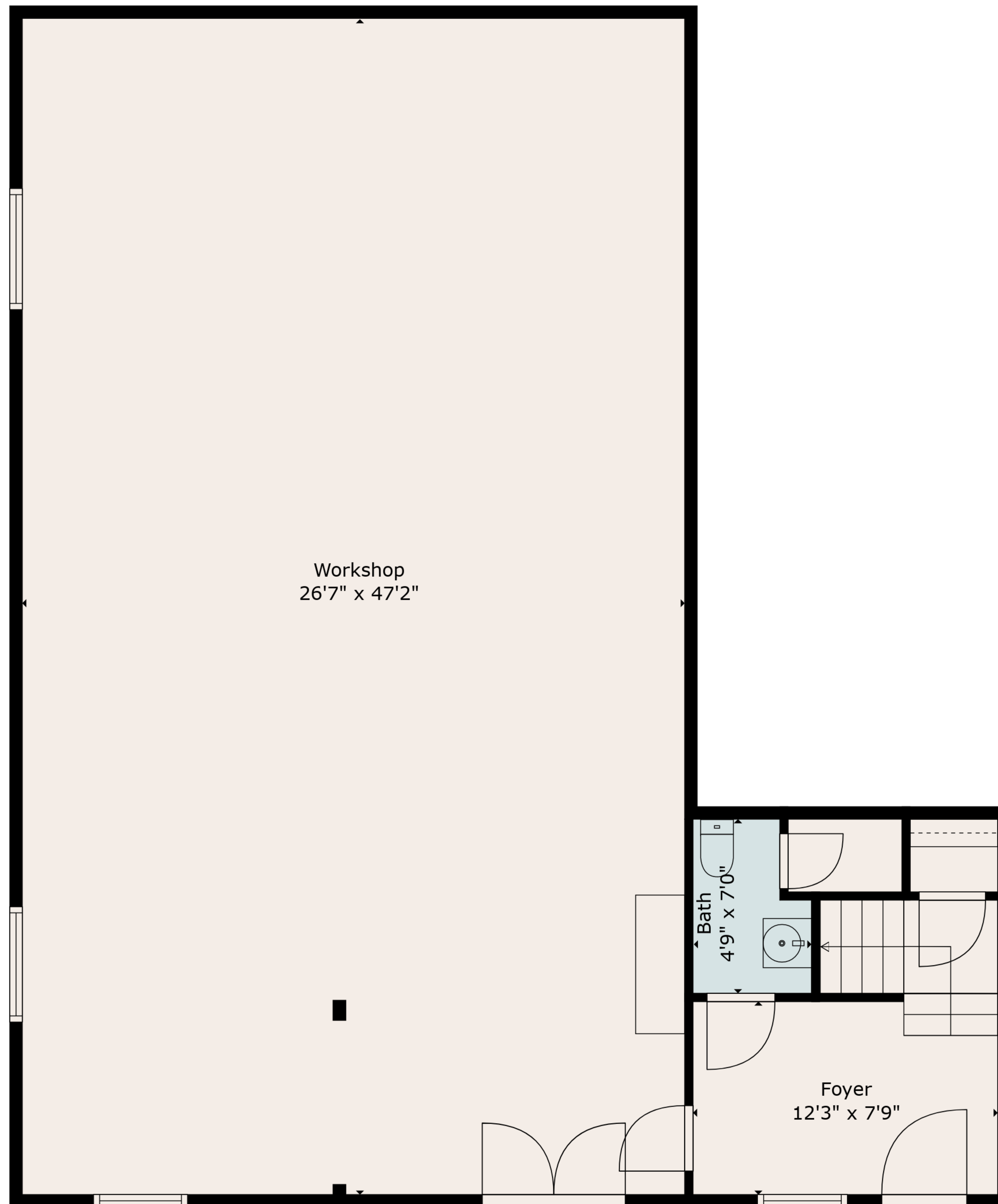
Floor 1
