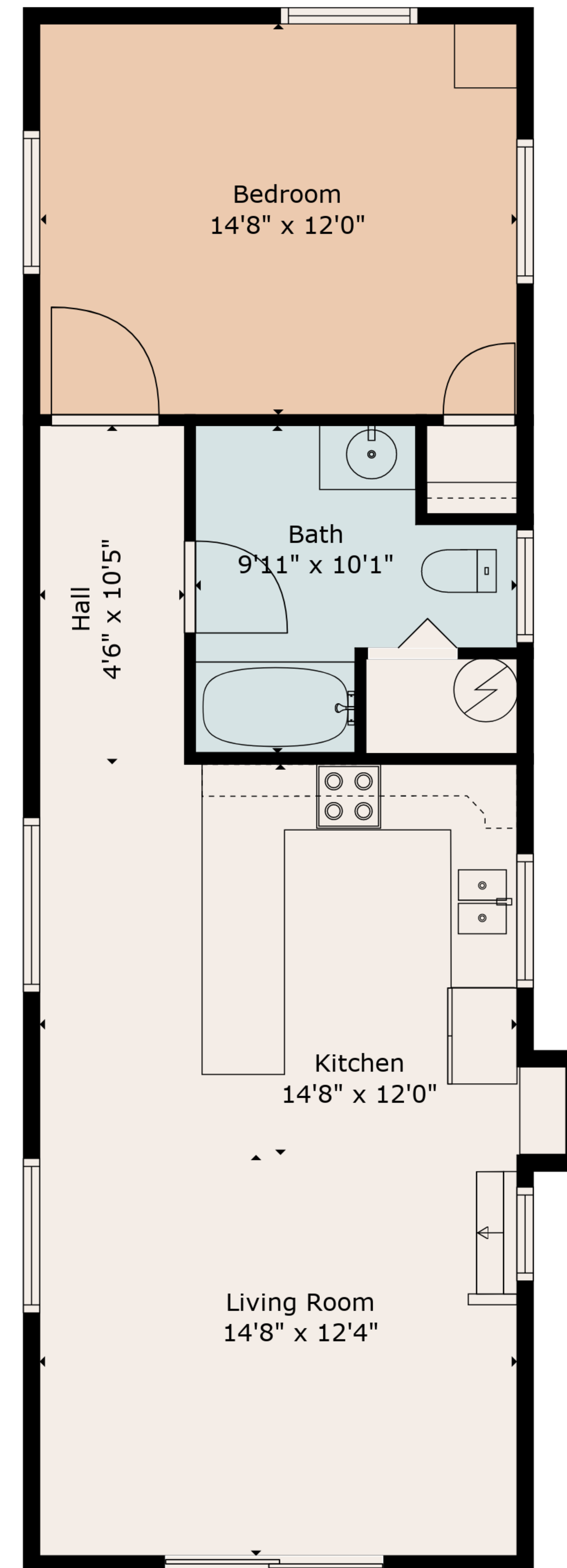
Floor 2
