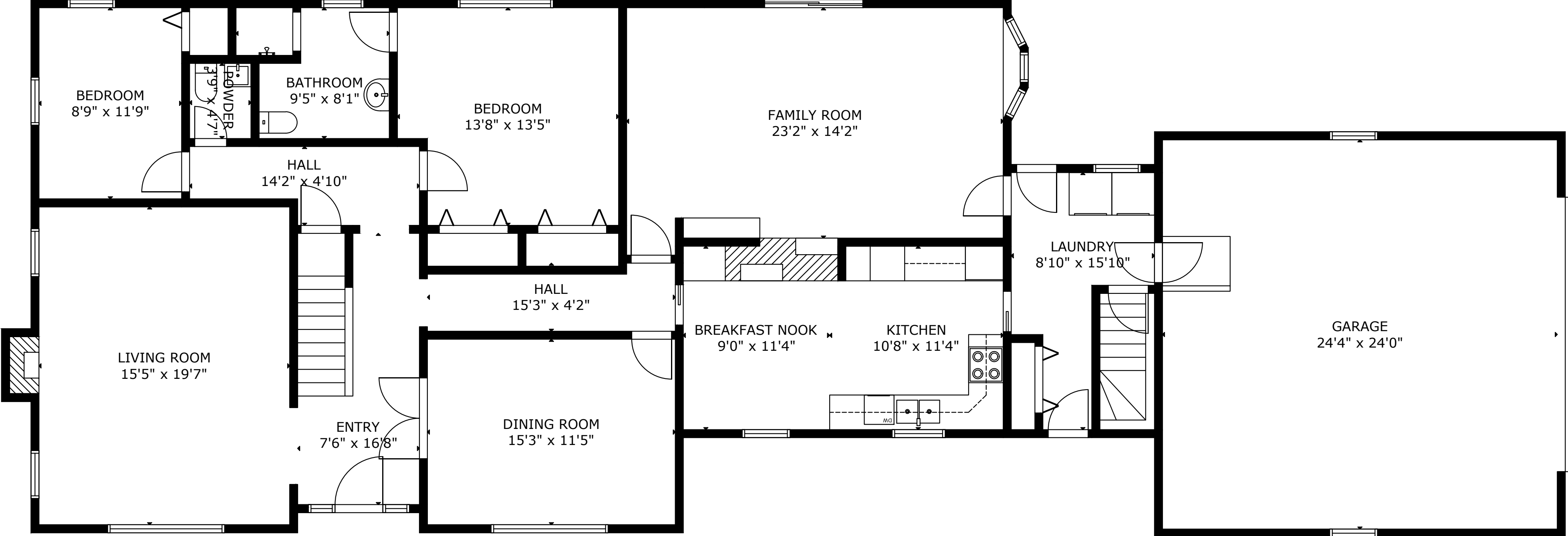
MAIN FLOOR
