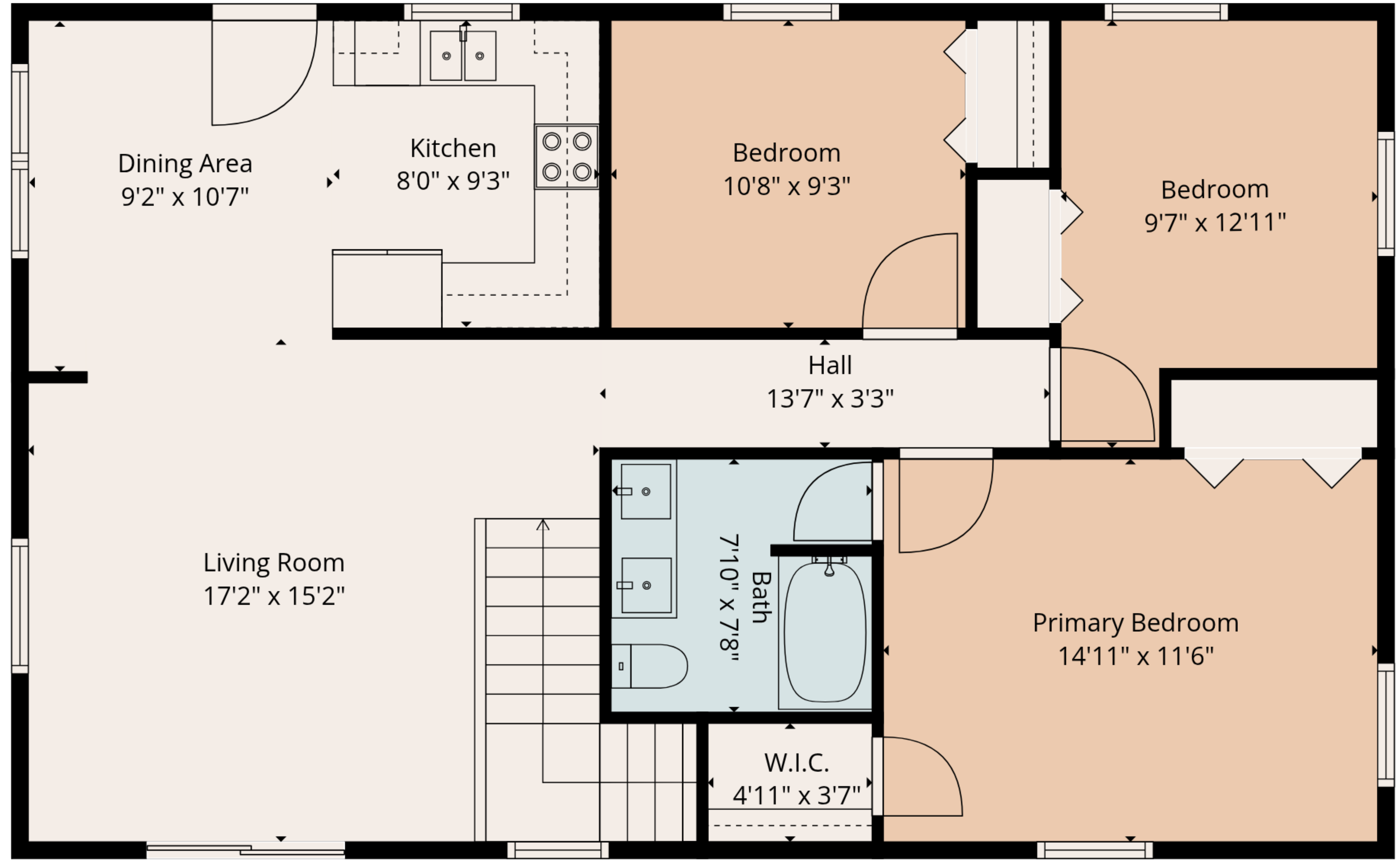
2nd Floor
