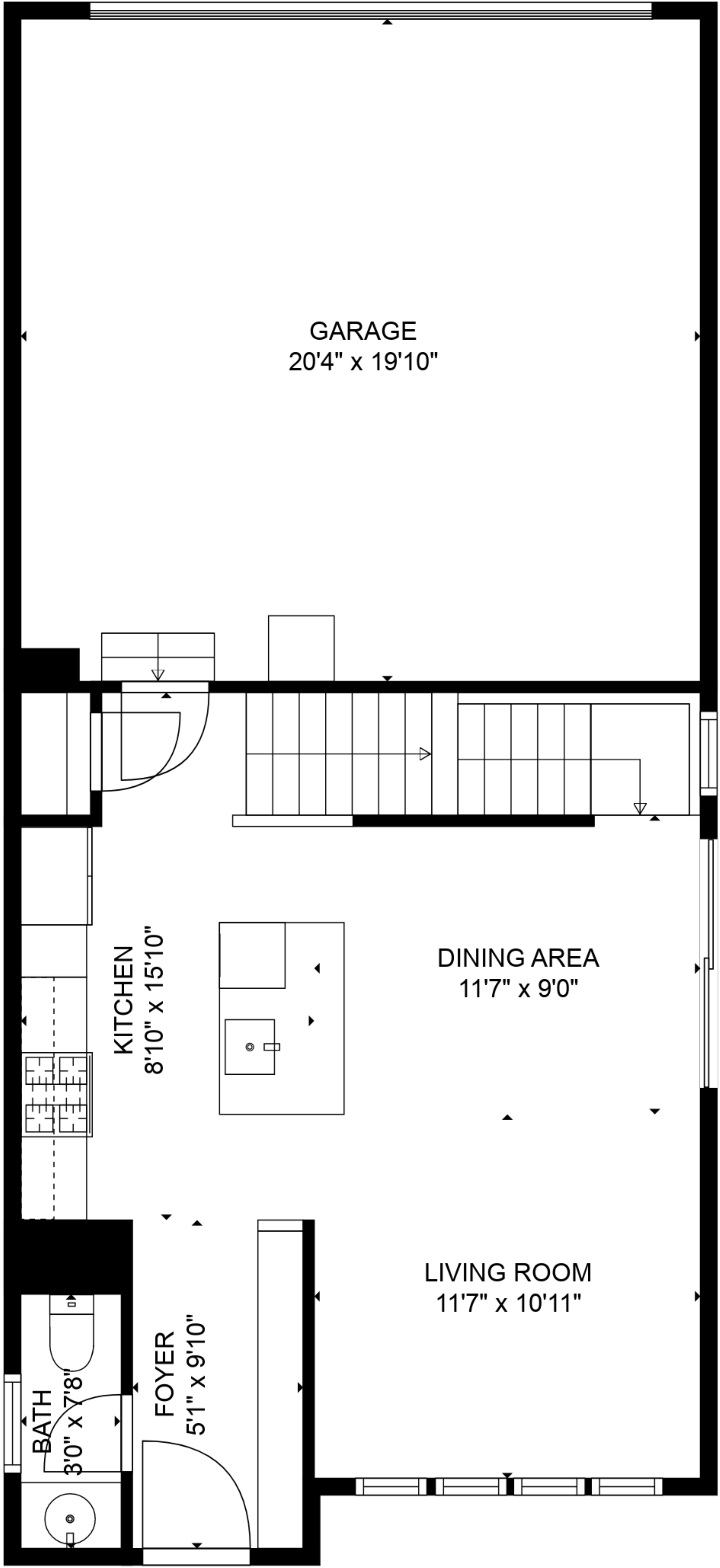
FLOOR 2
