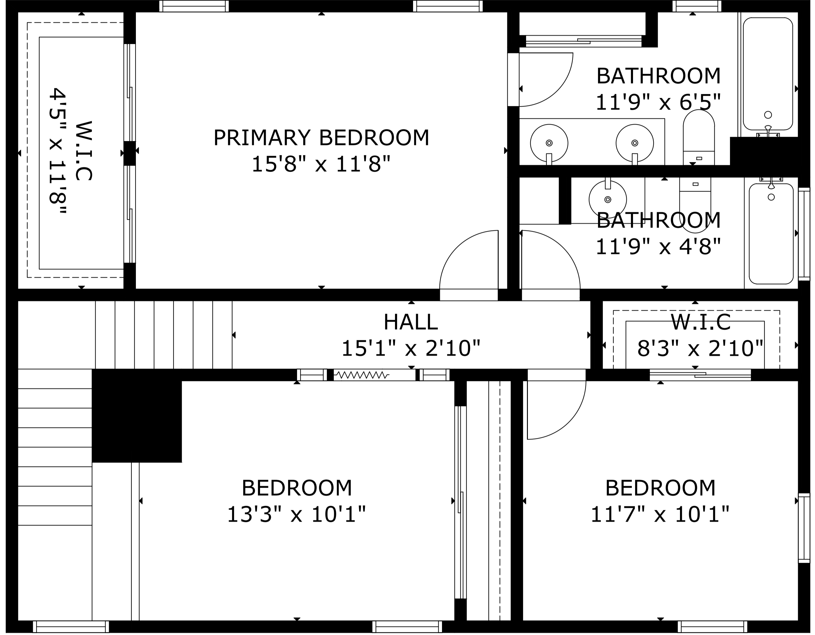
FLOOR 2
