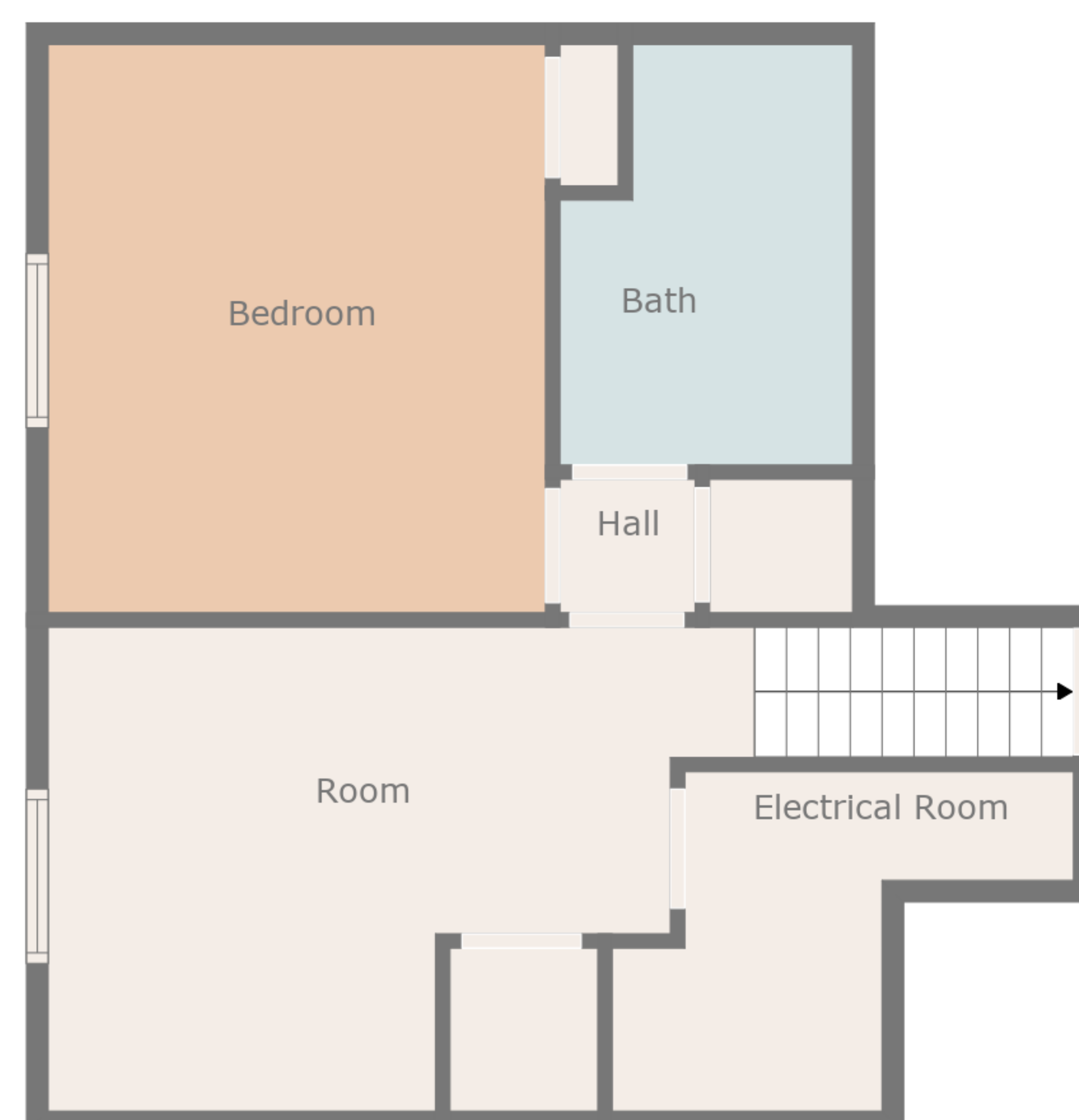
Floor 1
