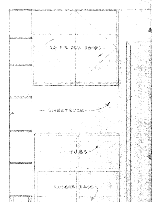
LAUNDRY - EAST WALL
