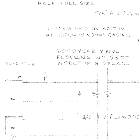
KITCHEN COUNTER DET.
