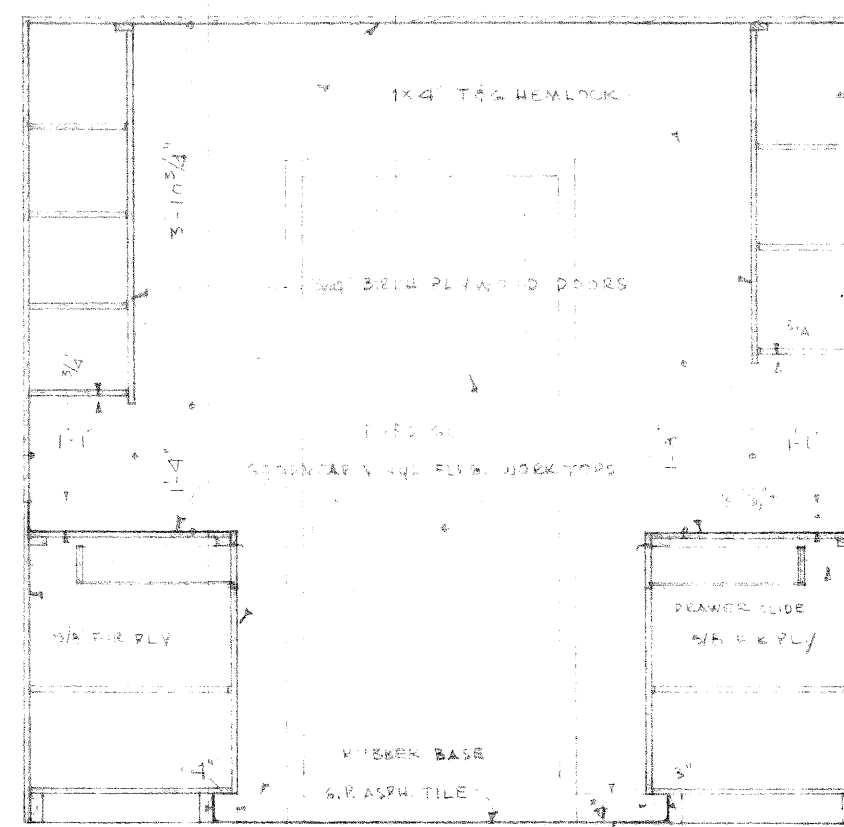
KITCHEN - WEST END
