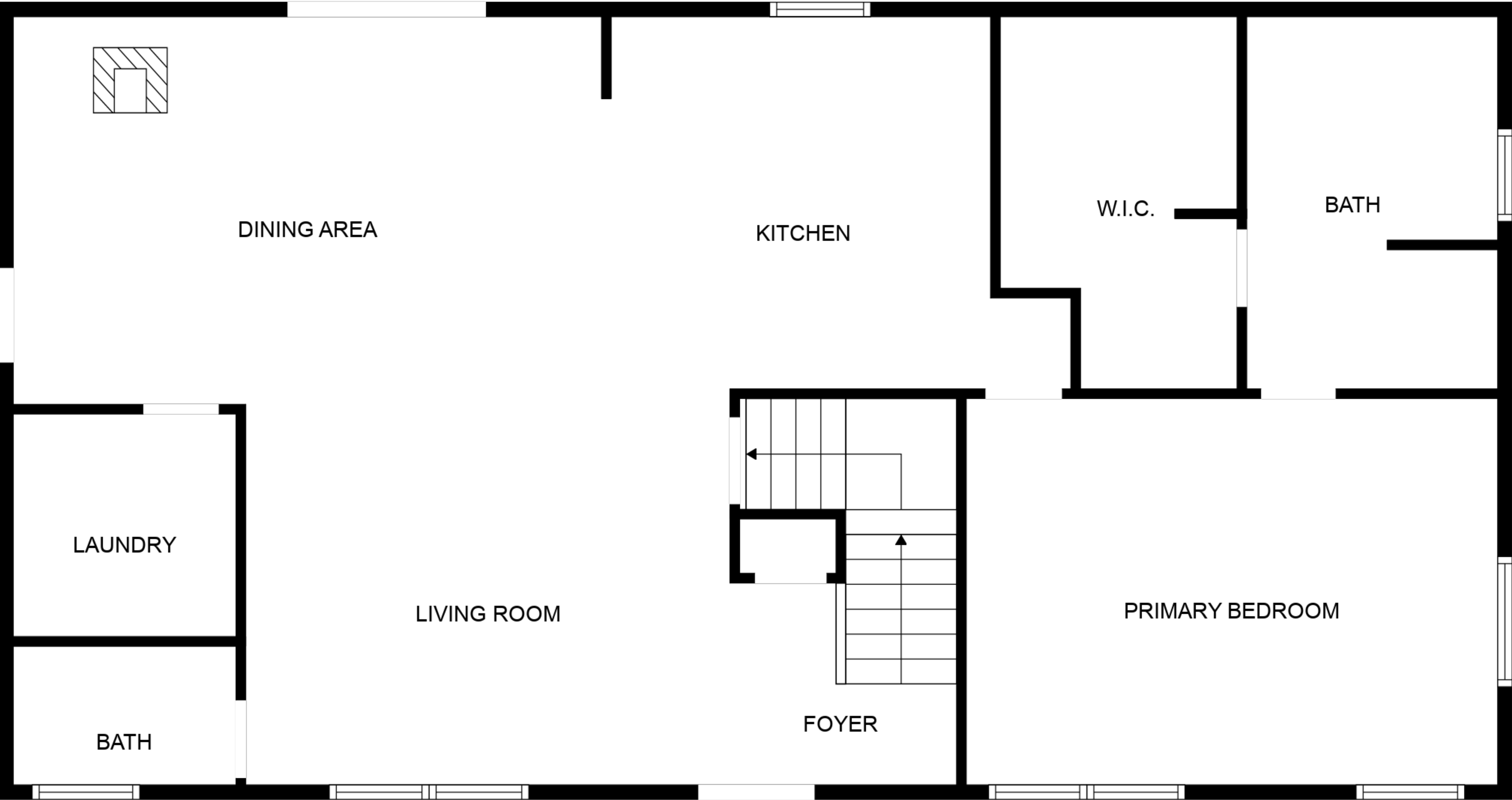
FLOOR 2
