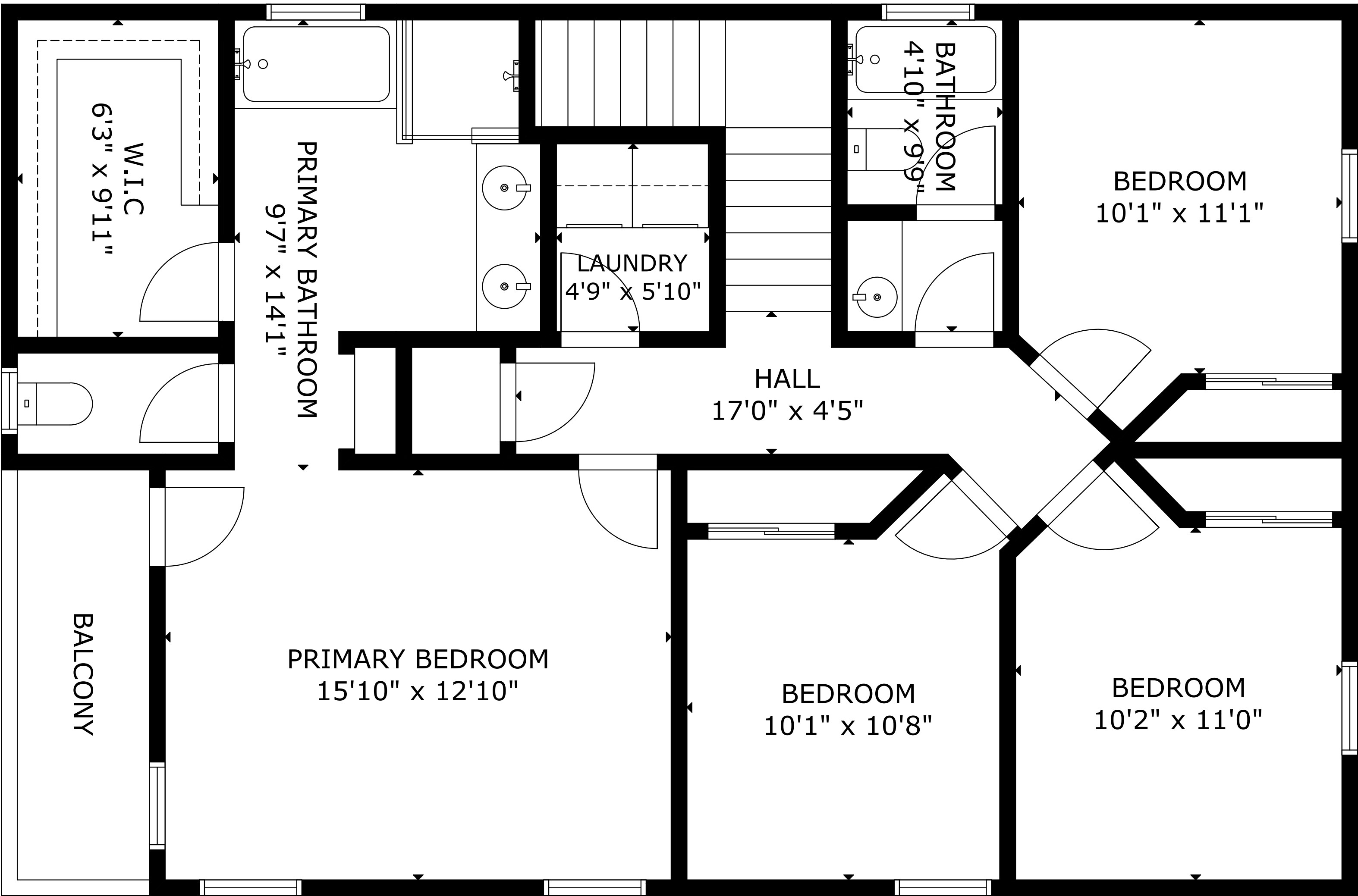
FLOOR 2
