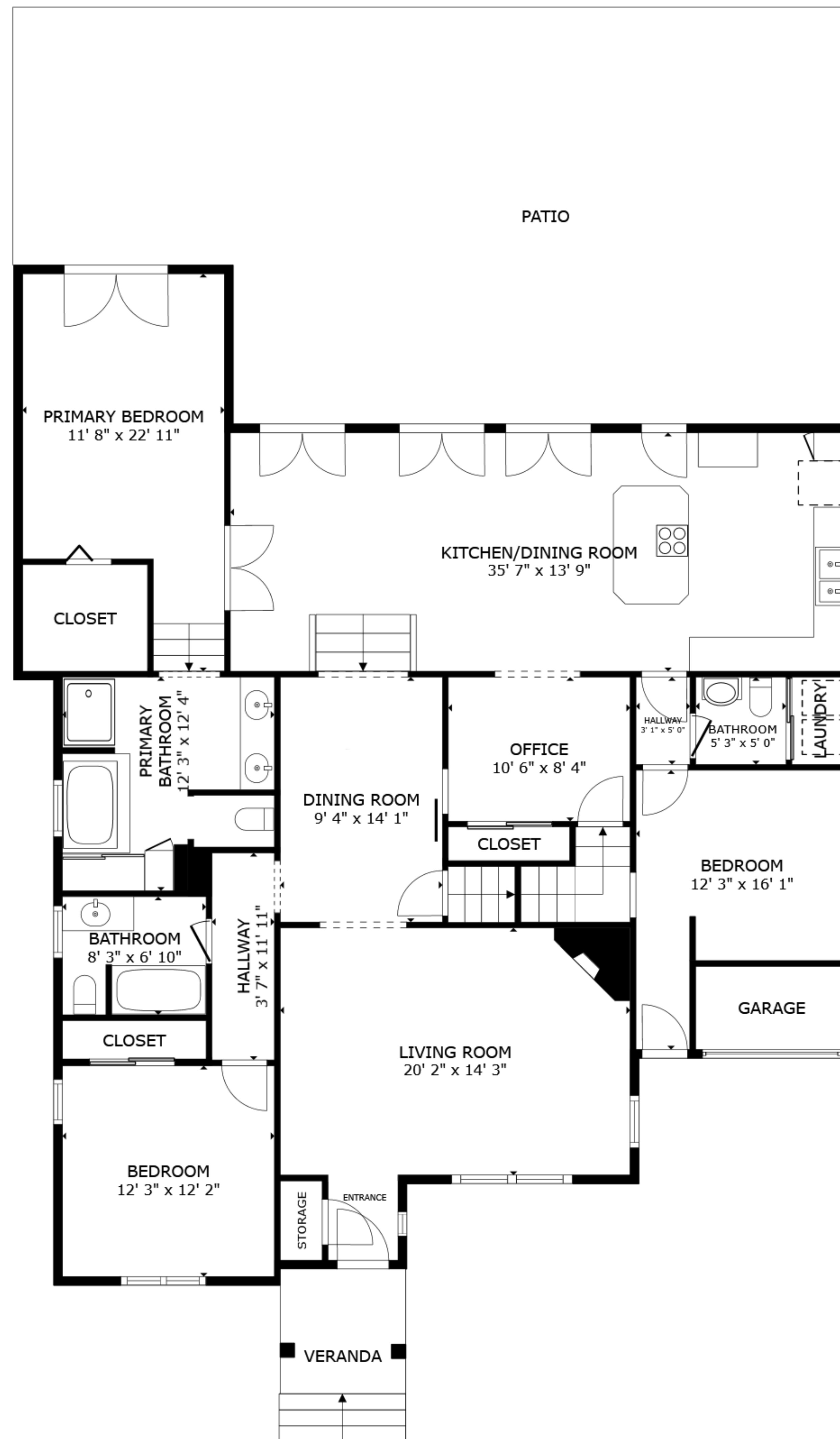
FLOOR 2
