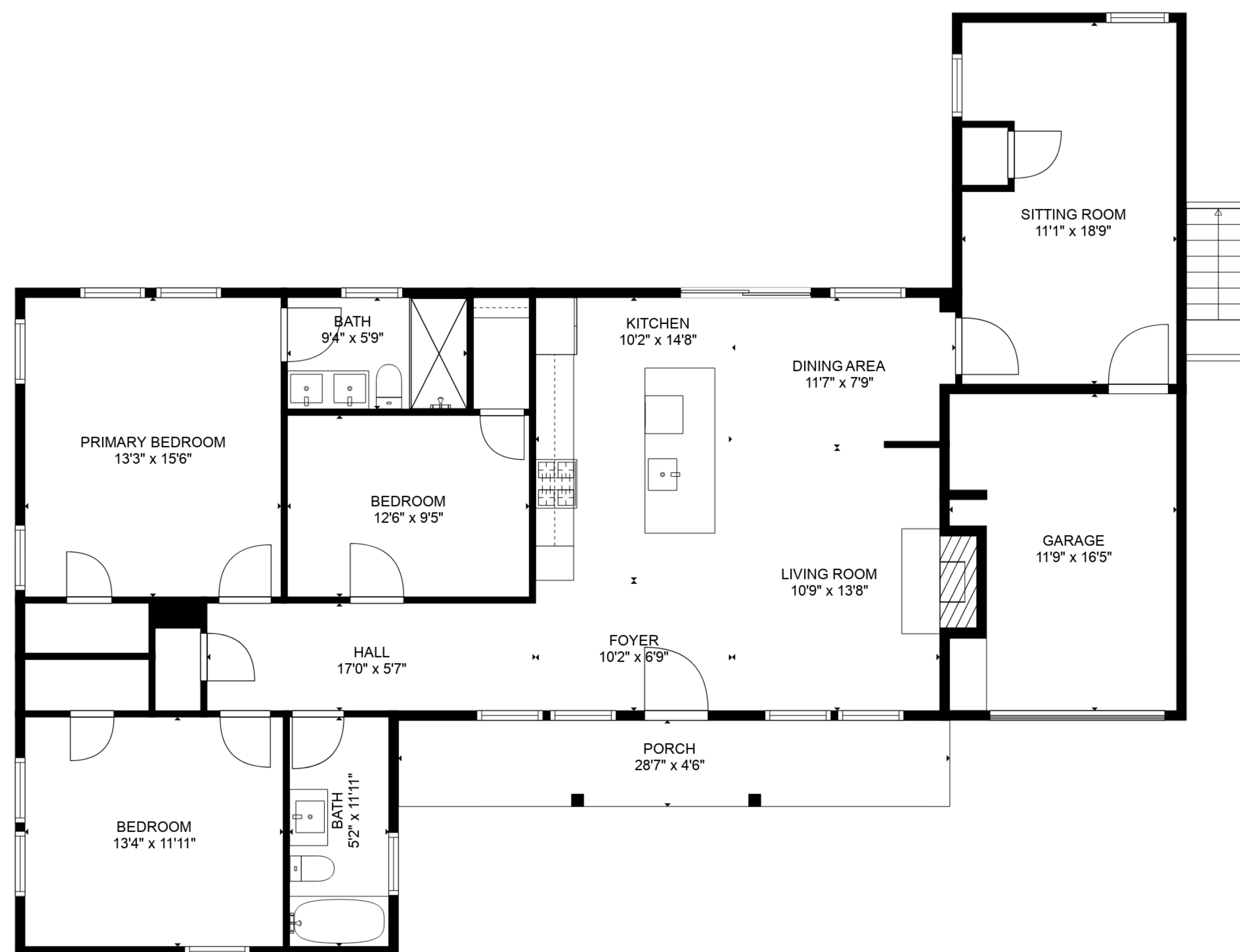
FLOOR 1
