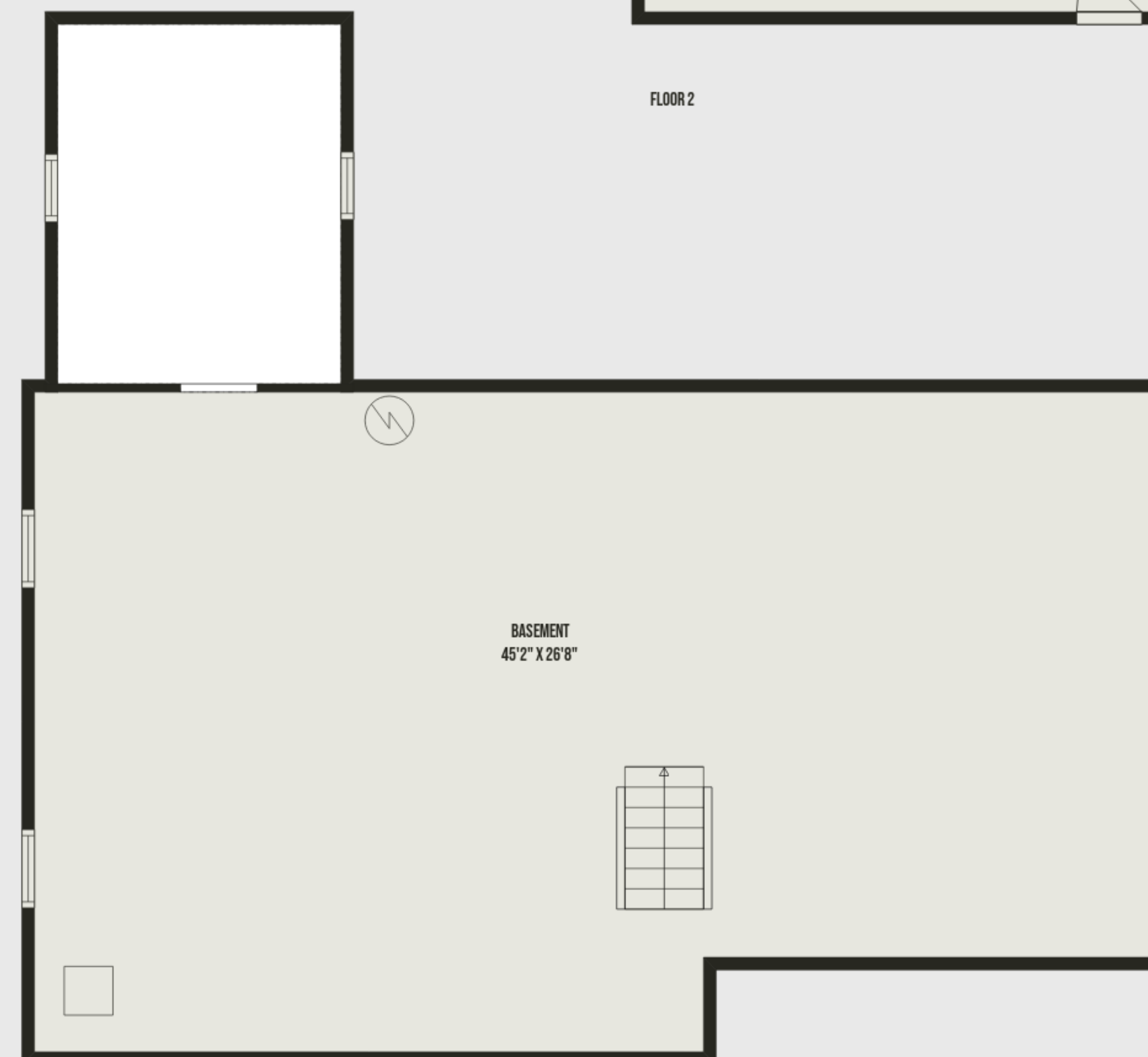
FLOOR 1
