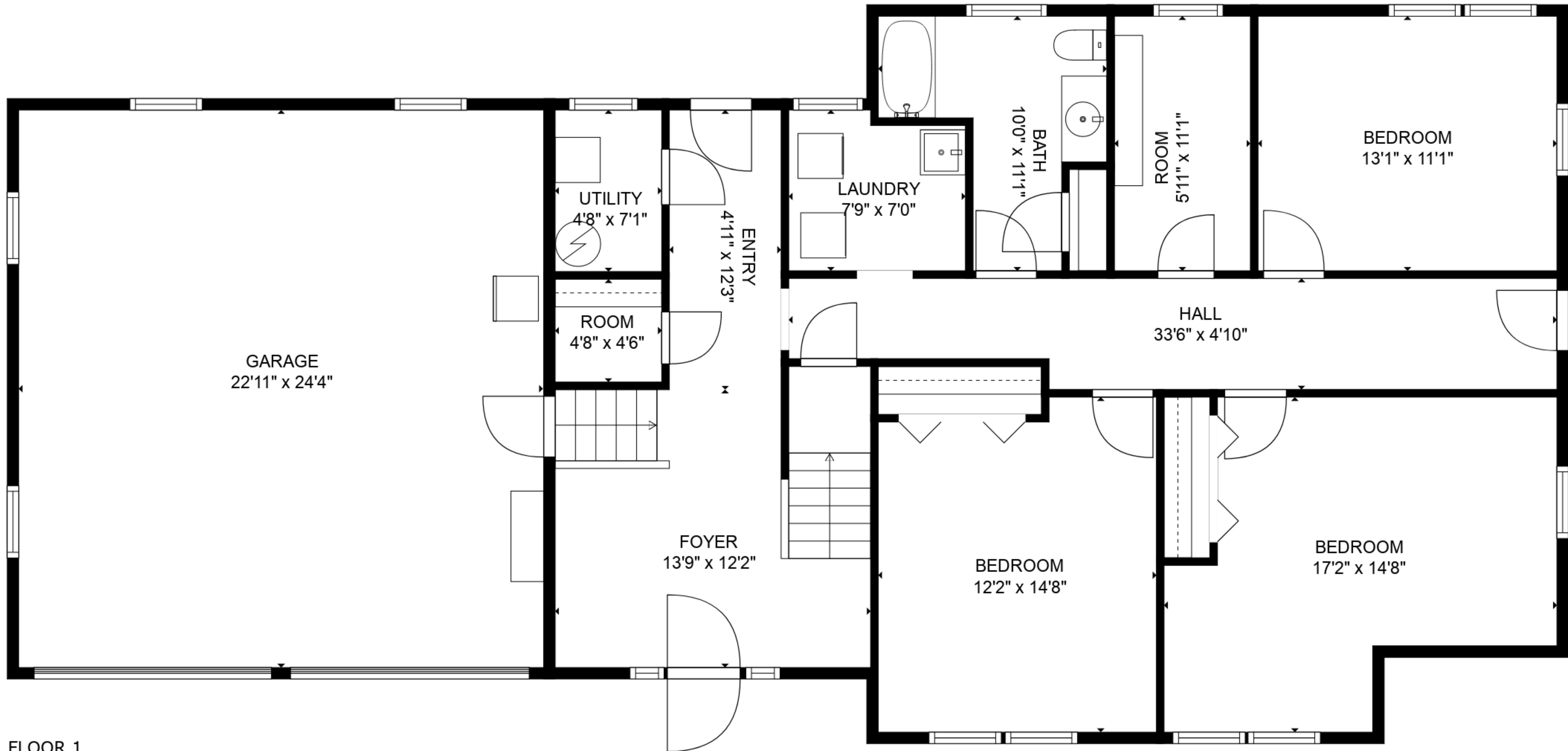
FLOOR 1
