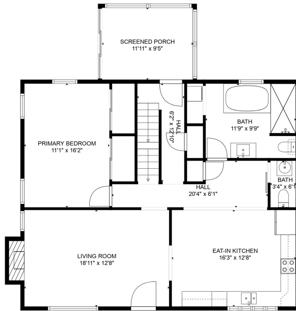
FLOOR 2
