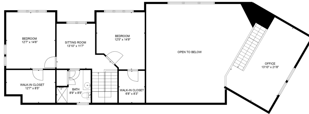
UPPER LEVEL
