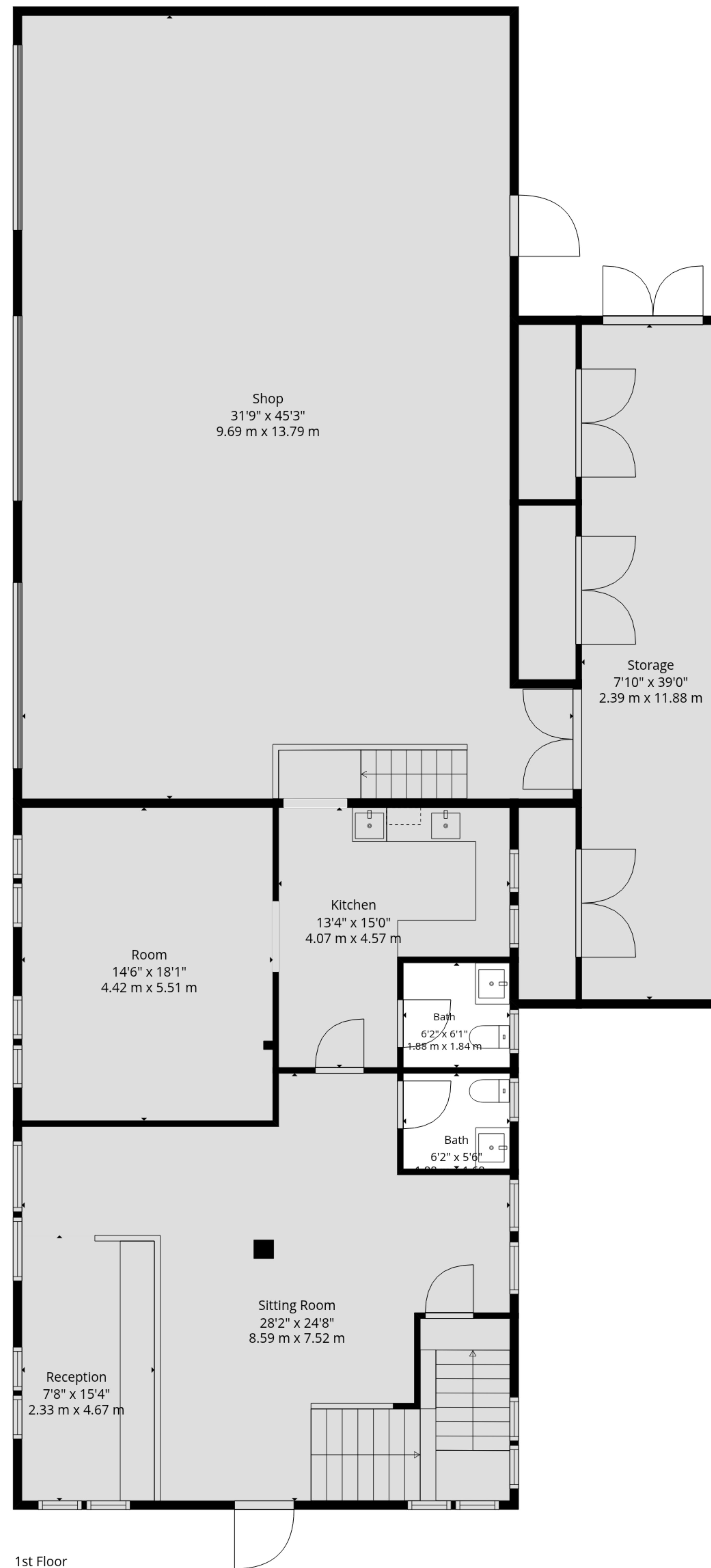
1st Floor
