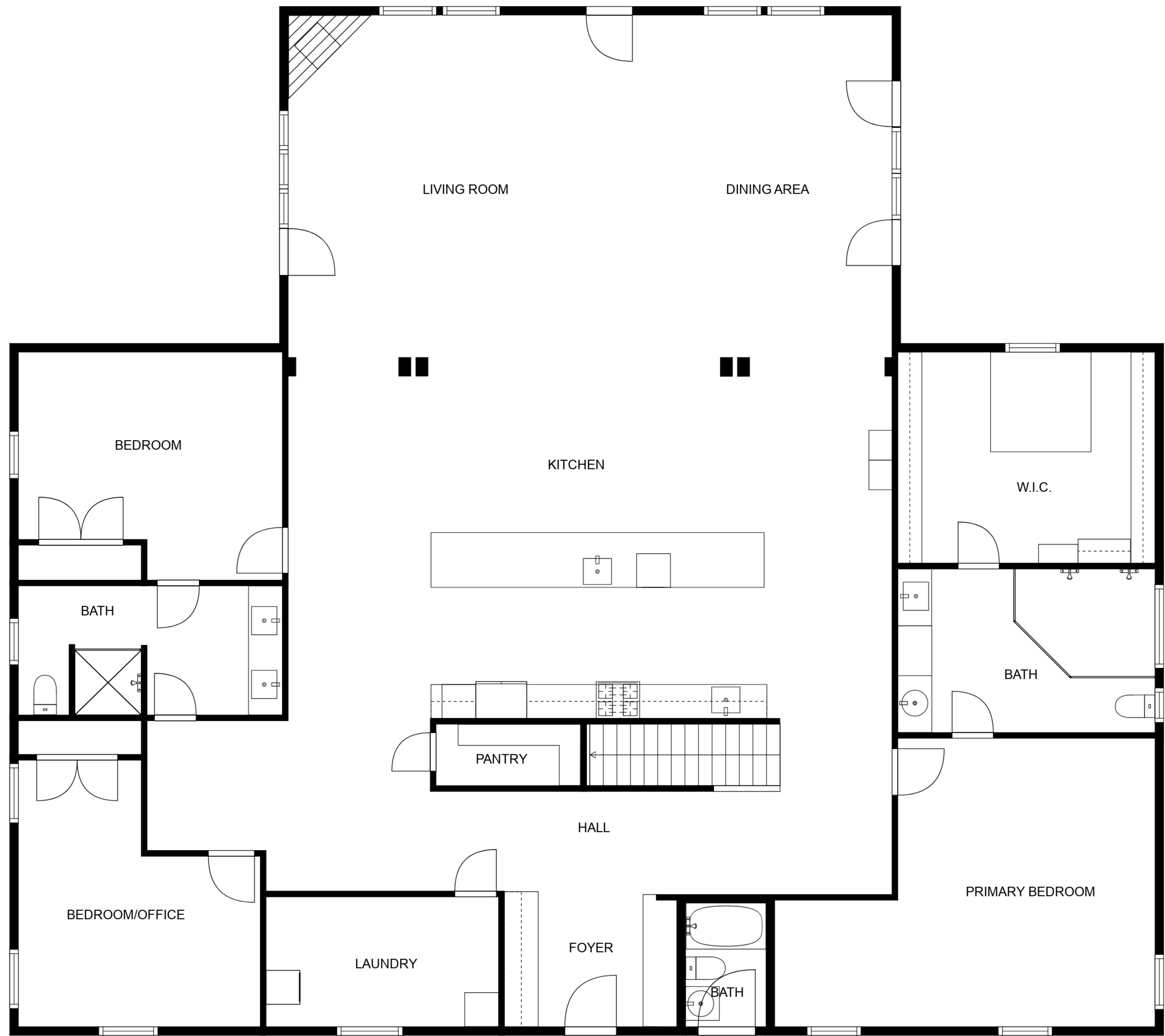
FLOOR 1
