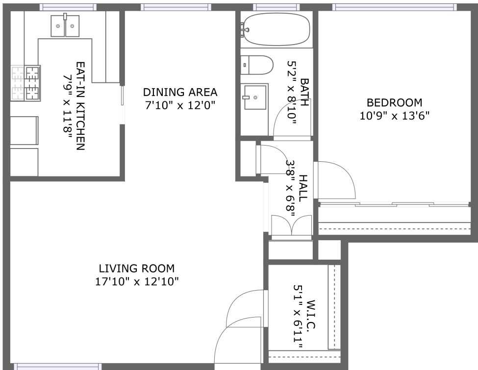
FLOOR 1
