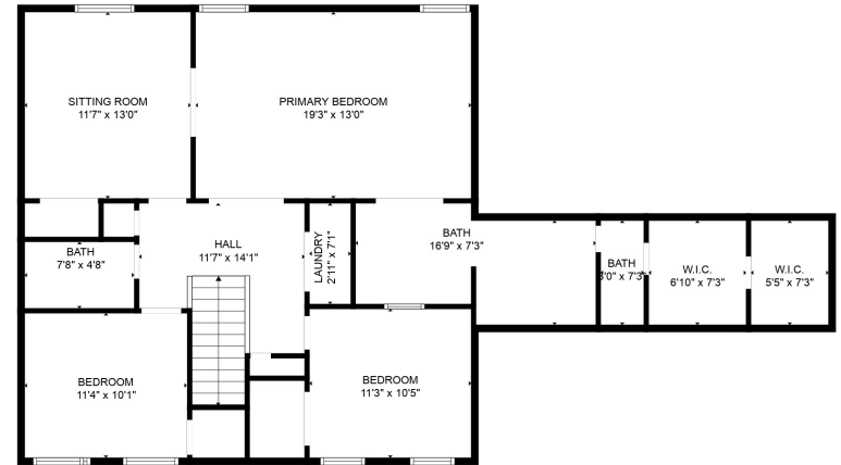
FLOOR 3
