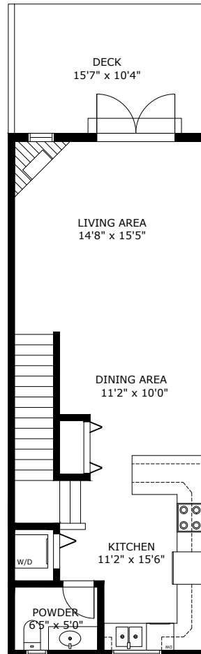
Main Level Area: Ceiling Height: 9'0"
