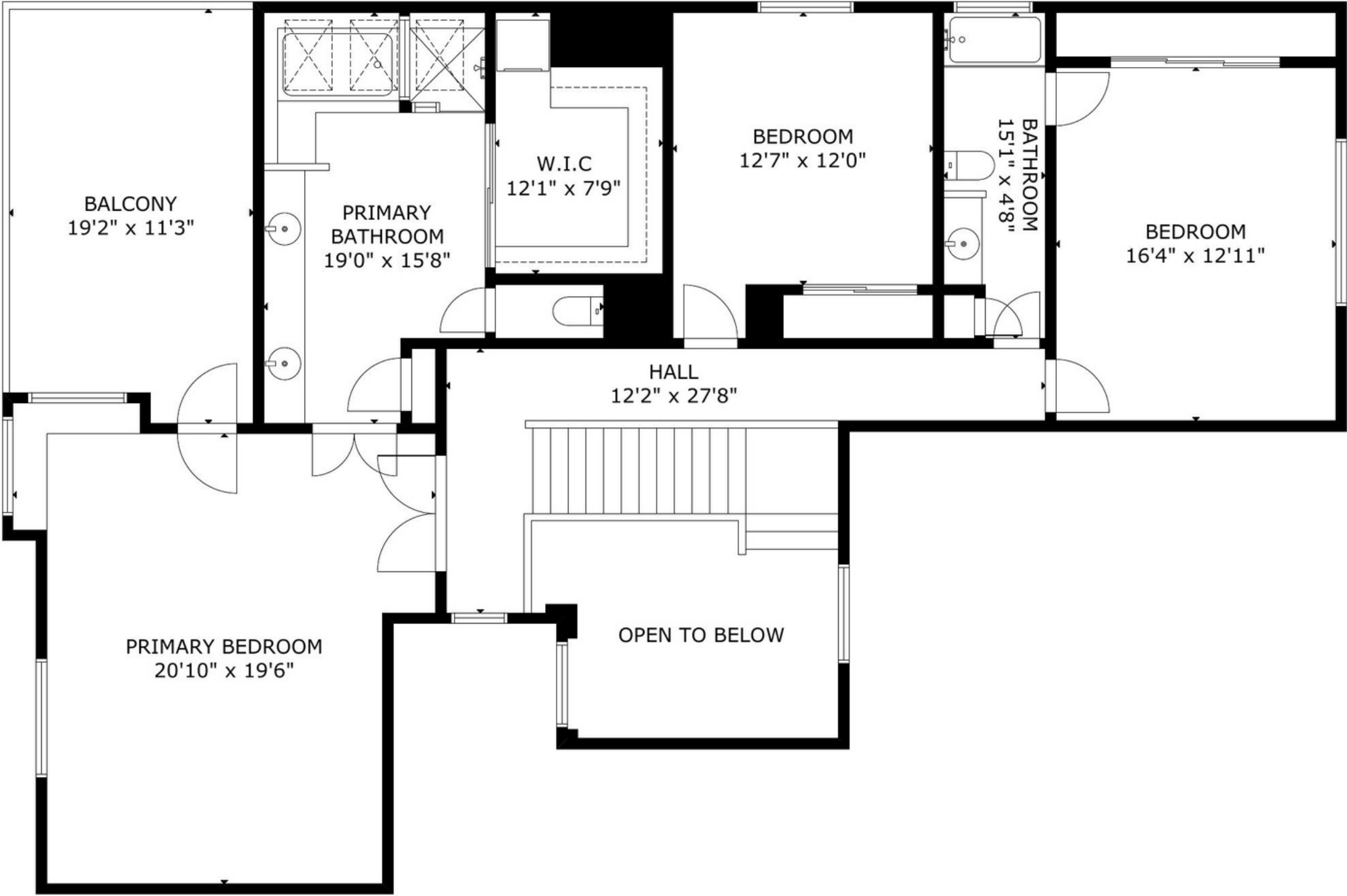
FLOOR 2
