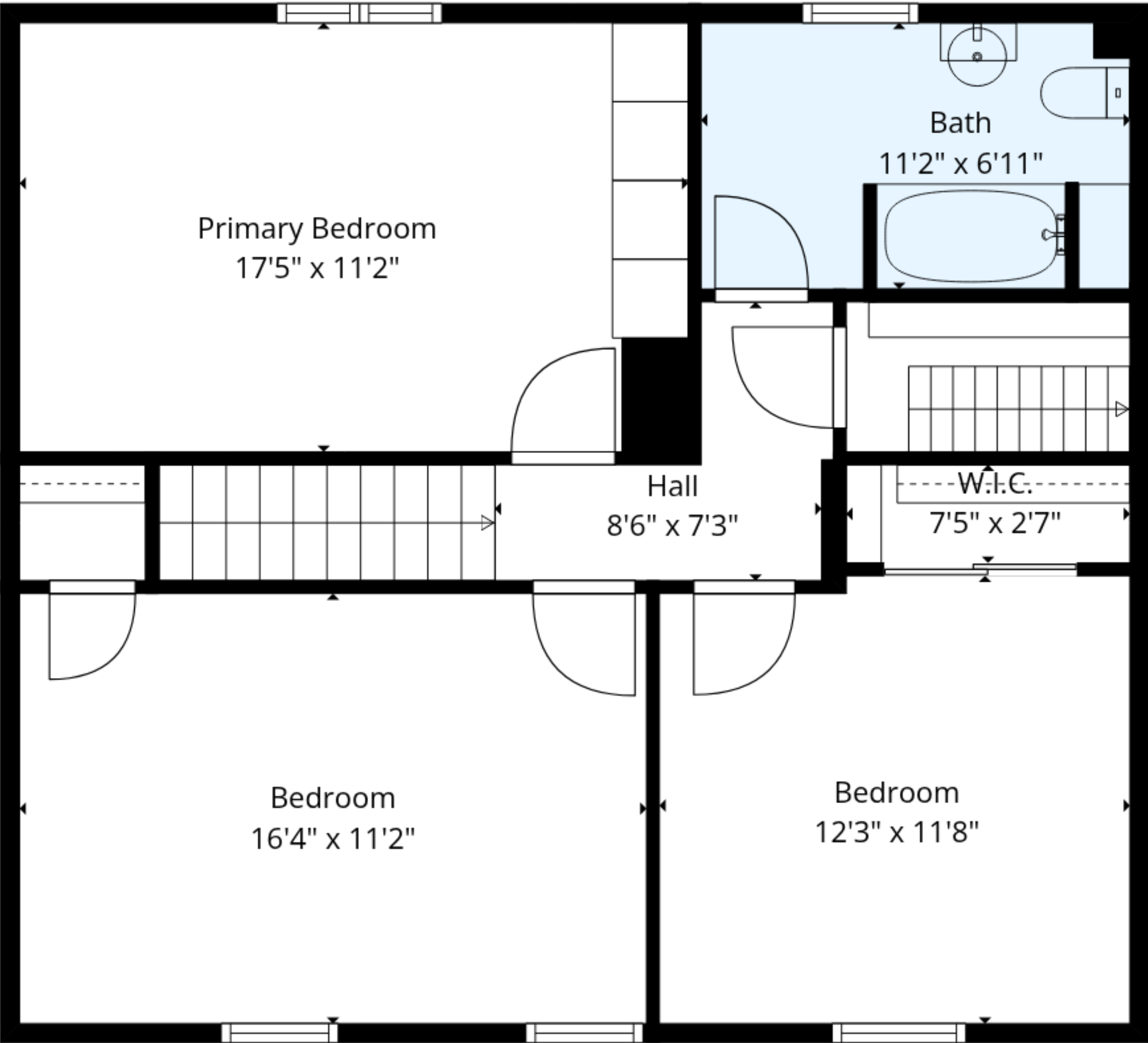
2nd Floor
