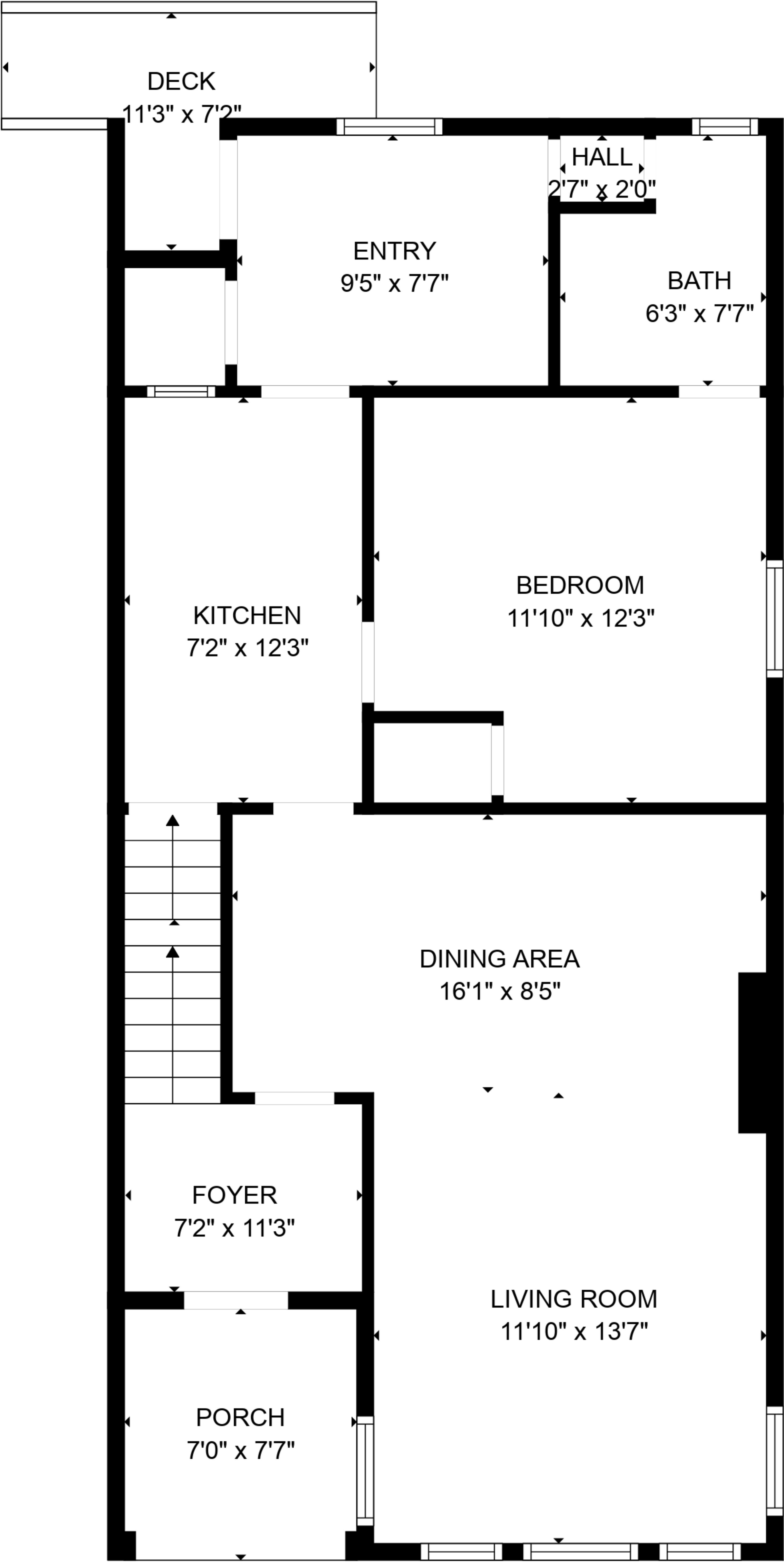
FLOOR 2
