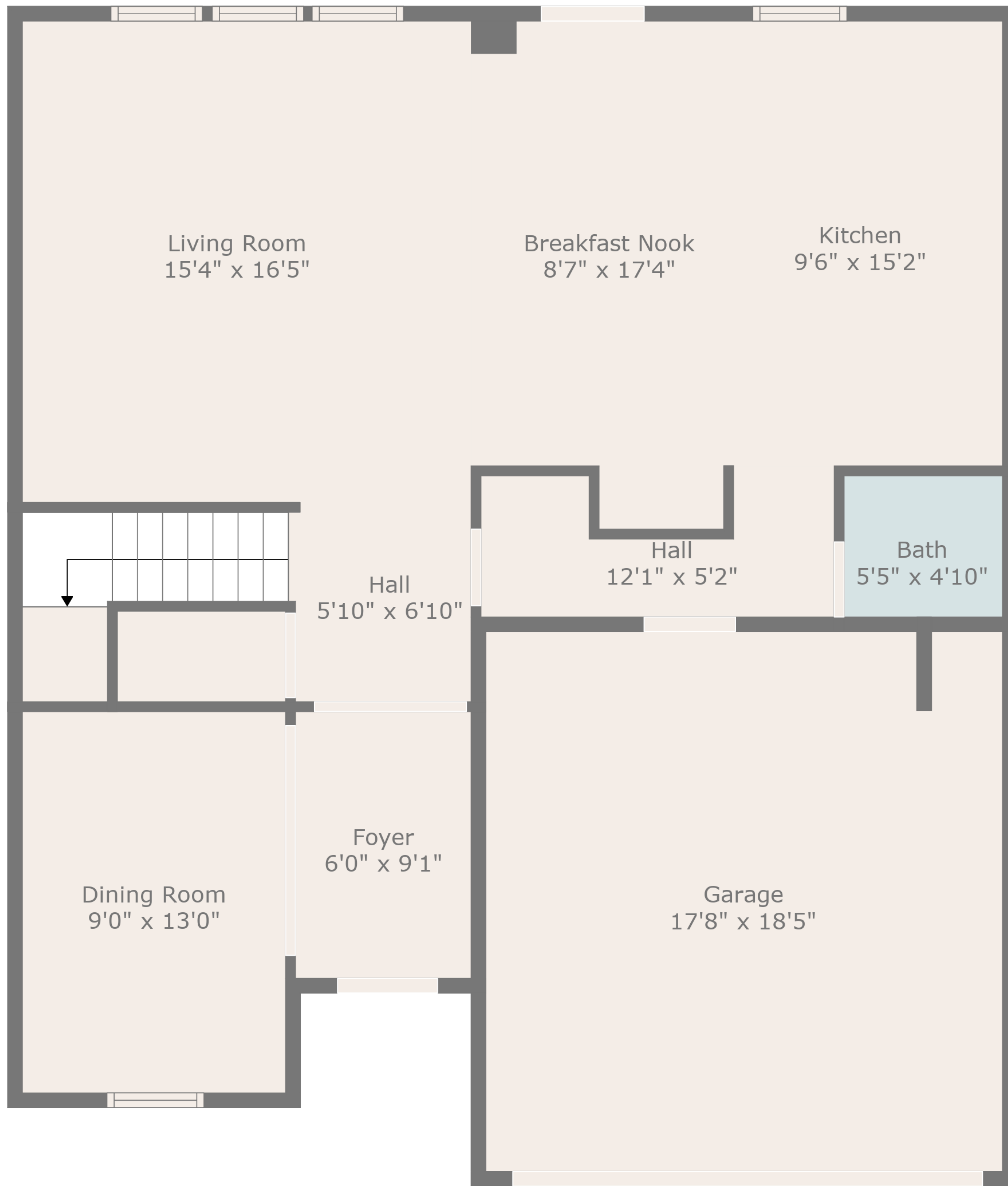
Floor 1
