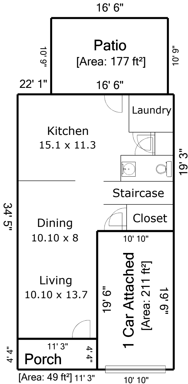
First Floor [Area: 596 ft²]
