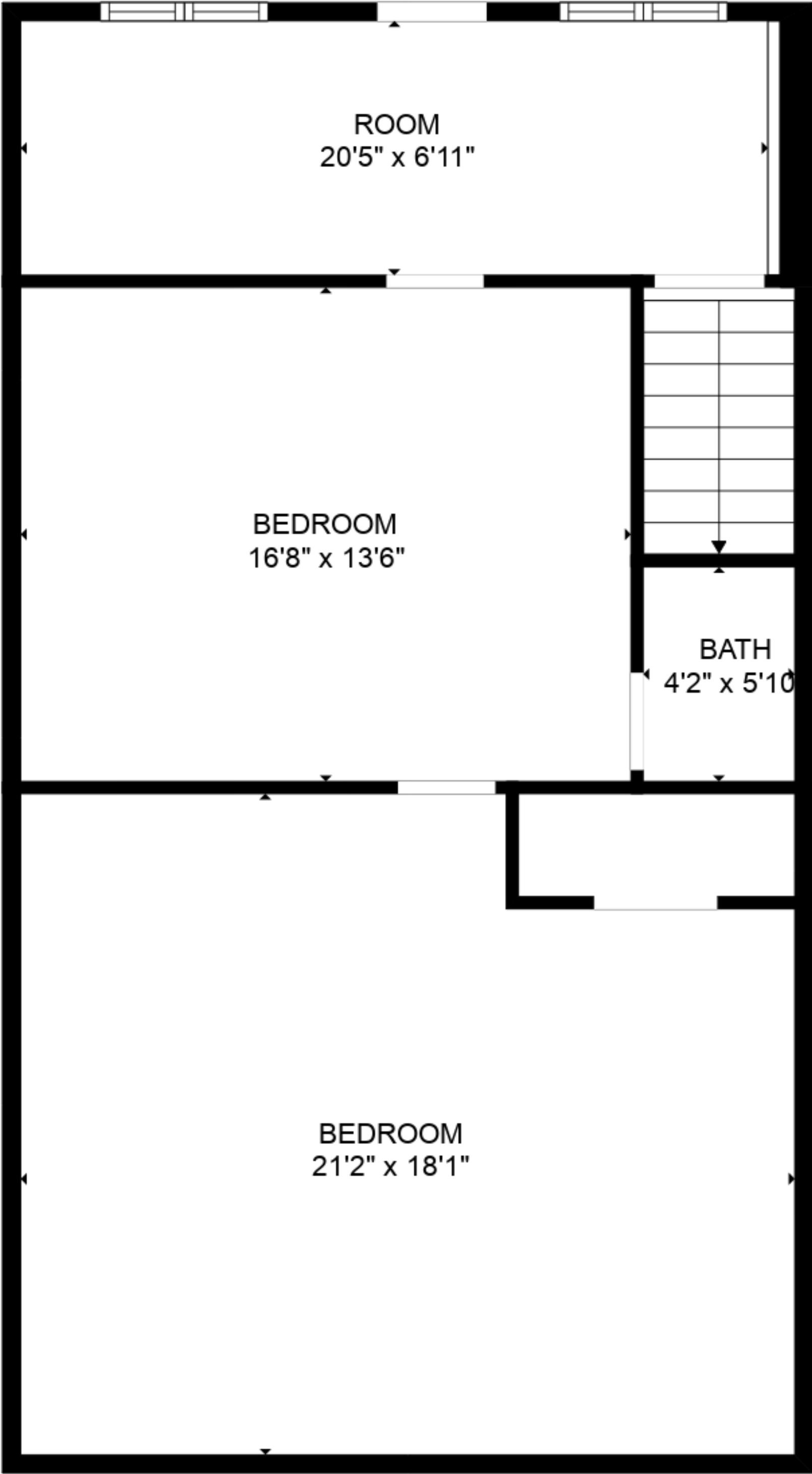
FLOOR 1
